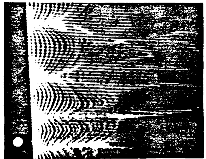
b) Turbulent boundary layer, Re_\theta = 2200 , y_{wire}^+ = 5
