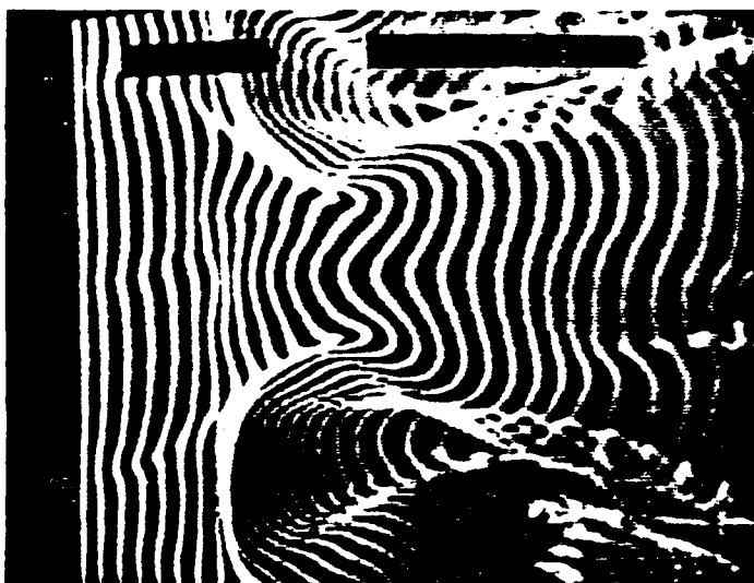
a) Hair-pin vortex, X/R = 20 , y_{wire}/R = 0.25
