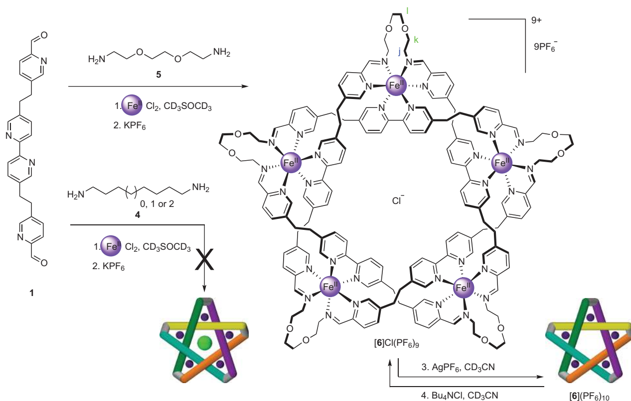
Figure 3 | Synthesis of molecular pentafoil knot [6]Cl(PF 6 ) 9 and 'empty cavity' pentafoil knot [6](PF 6 ) 10 . Reaction conditions: 1. d 6 -dimethylsulfoxide, 60 °C, 48 h. 2. Excess saturated aqueous KPF 6 . Yield of [6]Cl(PF 6 ) 9 from 1 , 44%. 3. AgPF 6 (90 equiv.), CD 3 CN, 30 min (>98%). 4. Bu 4 NCl (1 equiv.), CD 3 CN, 5 min (>98%).
