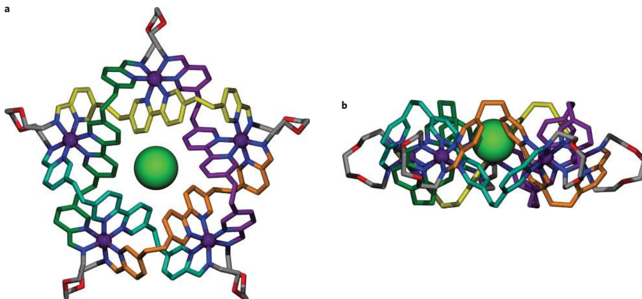
Figure 4 | X-ray crystal structure of molecular pentafoil knot [6]Cl(PF 6 ) 9 . Iron ions shown at 50% van der Waals radius. Chloride anion shown at 100% van der Waals radius. All other atoms shown in framework representation: nitrogen atoms, blue; oxygen atoms, red; carbon atoms originating from the diamine building block ( 5 ), grey; carbon atoms originating from the five dialdehyde building blocks ( 1 ), yellow, orange, dark green, purple and turquoise. PF 6 - anions, solvent molecules and hydrogen atoms are omitted for clarity. a , View from above the plane of the five octahedral Fe(II) ions, showing the symmetry and topology of the 160-atom-loop pentafoil knot with the chloride ion at the centre. CH δ+ ...Cl - distances (Å): 2.70, 2.69, 2.71, 2.70, 2.76, 2.76, 2.71, 2.70, 2.69, 2.76. C-H δ+ -Cl - angles (deg): 177, 176, 176, 172, 179, 173, 176, 170, 177, 170. O-C-C-O torsion angles (deg): 77(2), 64(3), 60(3), 56(3), 57(3). b , Side view showing the displacement of the chloride ion above the plane of the Fe(II) ions and the interwoven double helix of the ligand. Crystallographic data and experimental details of the structural refinement for [6]Cl(PF 6 ) 9 are provided in the Supplementary Information.
