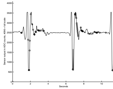
(b) Accelerometer 2
