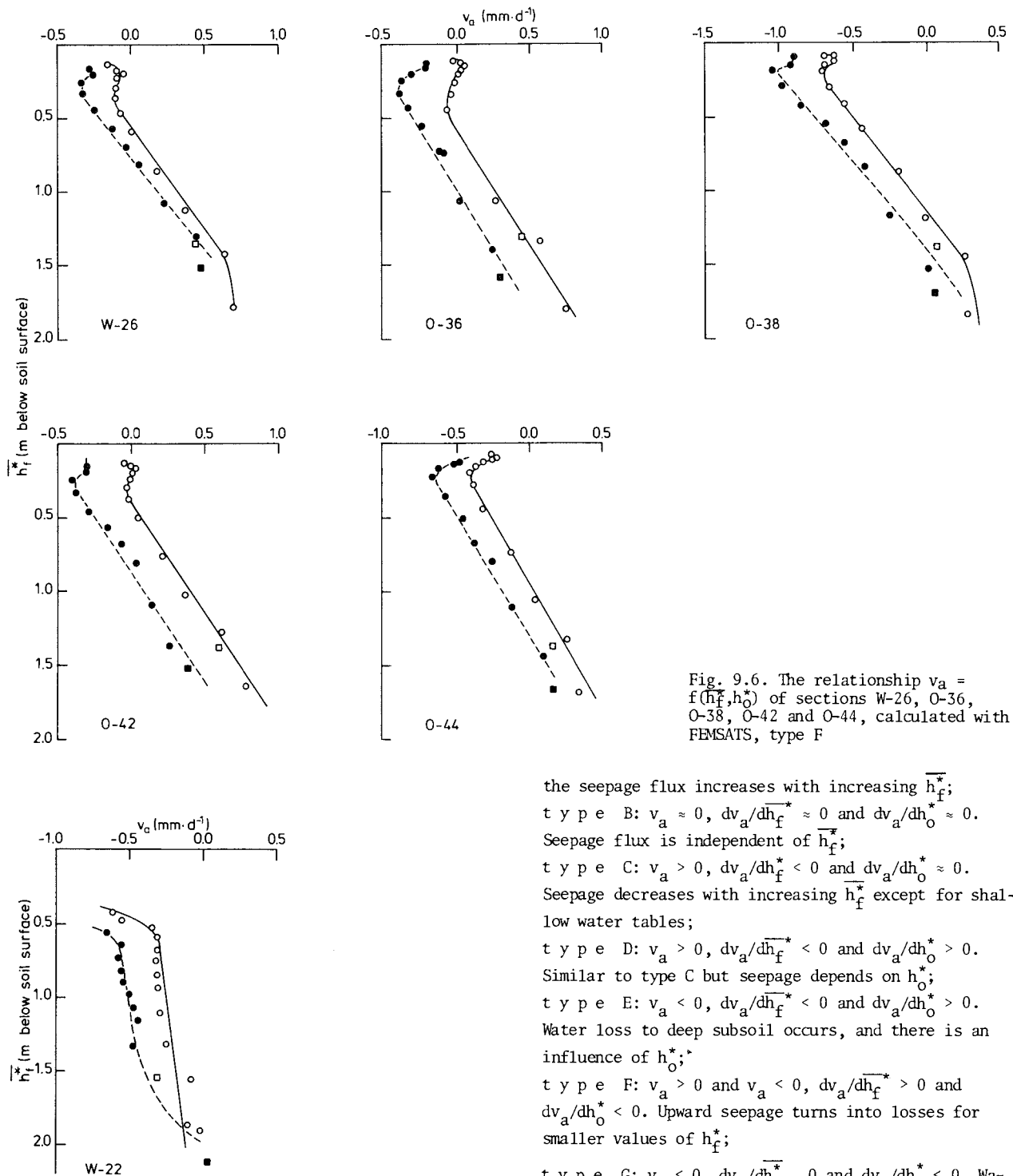
Fig. 9.7. The relationship v_a = f(\bar{h}_f^*, h_o^*) of section W-22, calculated with FEMSATS, type G
