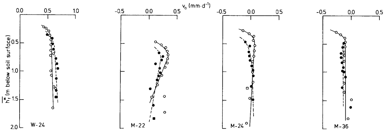
Fig. 9.2. The relationship v_a = f(\overline{h_f^*}, h_o^*) of sections W-24, M-22, M-24 and M-36, calculated with FEMSATS, type B
