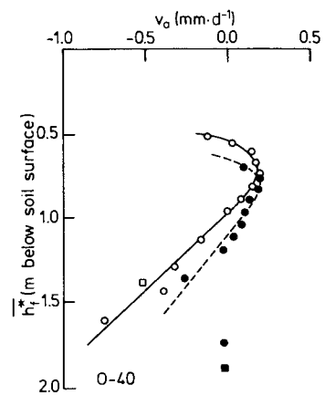
Fig. 9.5. The relationship v_a = f(\overline{h_f^*}, h_o^*) of section O-40, calculated with FEMSATS, type E
