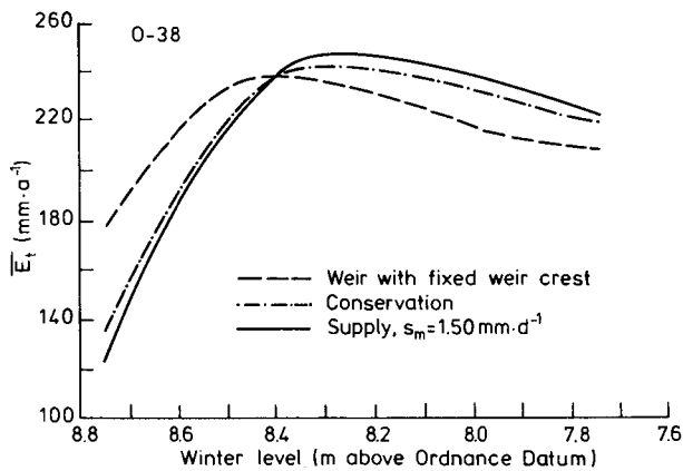
Fig. 9.9. Average yearly transpiration of potatoes, \bar{E}_t , of section O-38 derived from the relations in Fig. 9.8, for three alternative ways of surface water management
