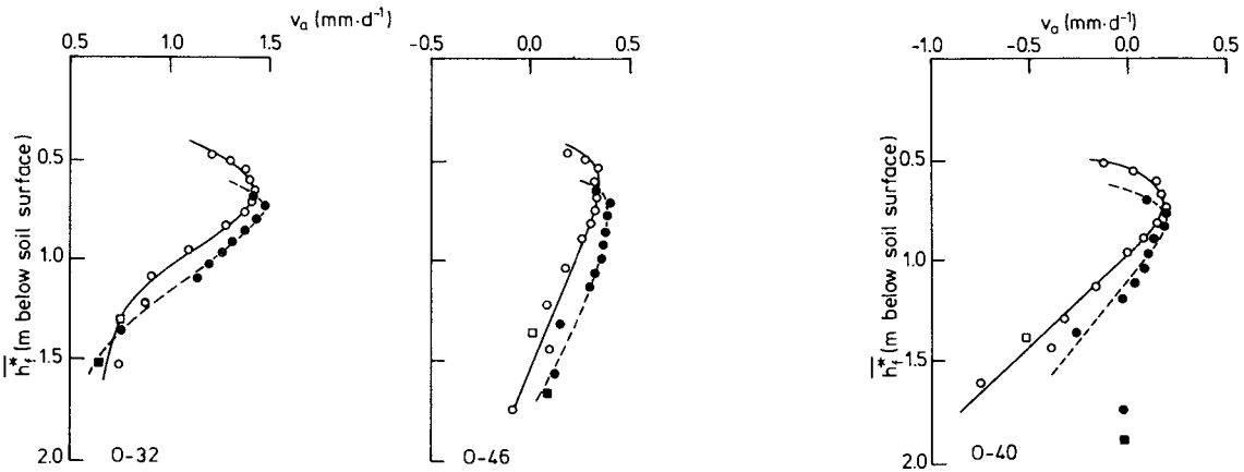
Fig. 9.4. The relationship v_a = f(\overline{h_f^*}, h_o^*) of sections O-32 and O-46, calculated with FEMSATS, type D
