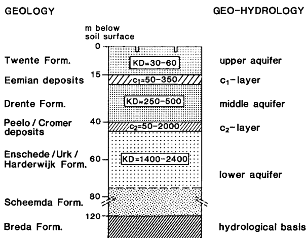
Fig. 4.4. Geo-hydrological schematization based on geological information
