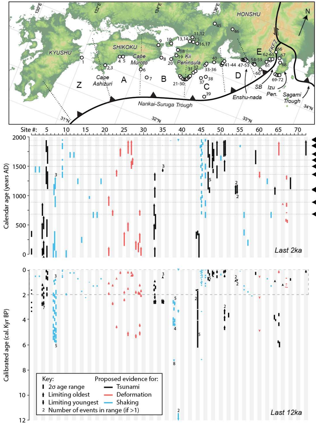
Figure 3: Summary of the spatial and temporal distribution of proposed evidence for past megathrust earthquakes along the Nankai-Suruga Trough. We emphasise that for many of the records summarised here, alternative, non-seismic formation mechanisms are yet to be discounted. Upper panel displays site locations, lower panels give age ranges and limiting dates for proposed palaeoseismic evidence. Site numbers: 1 Ryūjin Pond*; 2 Azono*; 3 Funato*; 4 Tadasu Pond†; 5 Kani Pond*; 6 Cape Muroto; 7 Tosabae Trough‡; 8 Kamoda Lake*; 9 Itano-chō*; 10 Shimonaizen*; 11 Kosaka-tei-ato*; 12 Ikeshima Fukumanji*; 13 Iwatsuta Shrine*; 14 Sakai-shi Shimoda*; 15 Tainaka*; 16 Hashio*; 17 Sakafuneishi*; 18 Kawanabe*; 19 Fujinami*; 20 Hidaka Marsh§; 21 Kuchiwabuka†; 22 Ameshima†; 23 Shionomisaki†; 24 Izumozaki†; 25 Arafunezaki†; 26
