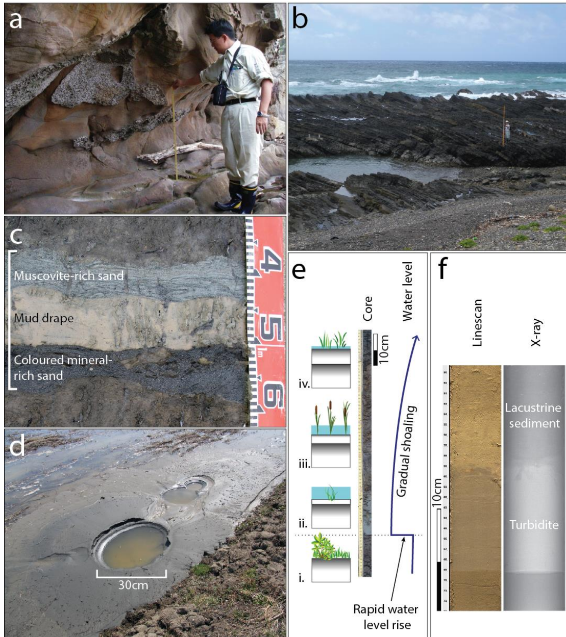
Figure 2: Representative photographs of different lines of palaeoseismic evidence that have been employed along the Nankai-Suruga Trough. a) Emerged sessile organisms at Suzushima close to the boundary between segments B and C. Mass mortality of colonies of intertidal annelid worms reflects coseismic uplift during an earthquake approximately 2000 cal. yr BP (Shishikura et al., 2008). b) An emerged wave cut platform near Cape Ashizuri. The platform lies at an elevation of approximately 1 – 1.2 m above present mean sea level and may reflect uplift during the AD 1946 earthquake (M. Shishikura, unpublished data). c) Layers of sand and mud probably left by the AD 1605 tsunami at Shirasuka (Fujiwara et al., 2006). d) Liquefaction features (sand blows) induced by intense shaking during the 2011 Tōhoku earthquake (O. Fujiwara, unpublished data). e) An abrupt transition from peat to tidal flat mud resulting from coseismic subsidence of the Ukishima-ga-hara Lowlands in segment E (Fujiwara et al., 2016). Peat accumulating on a marsh (i.) is abruptly overlain by inorganic mud (ii.) after a rapid rise in water level, followed by a gradual return to organic sedimentation and the recovery of the marsh (iii. and iv.). f) A lacustrine
