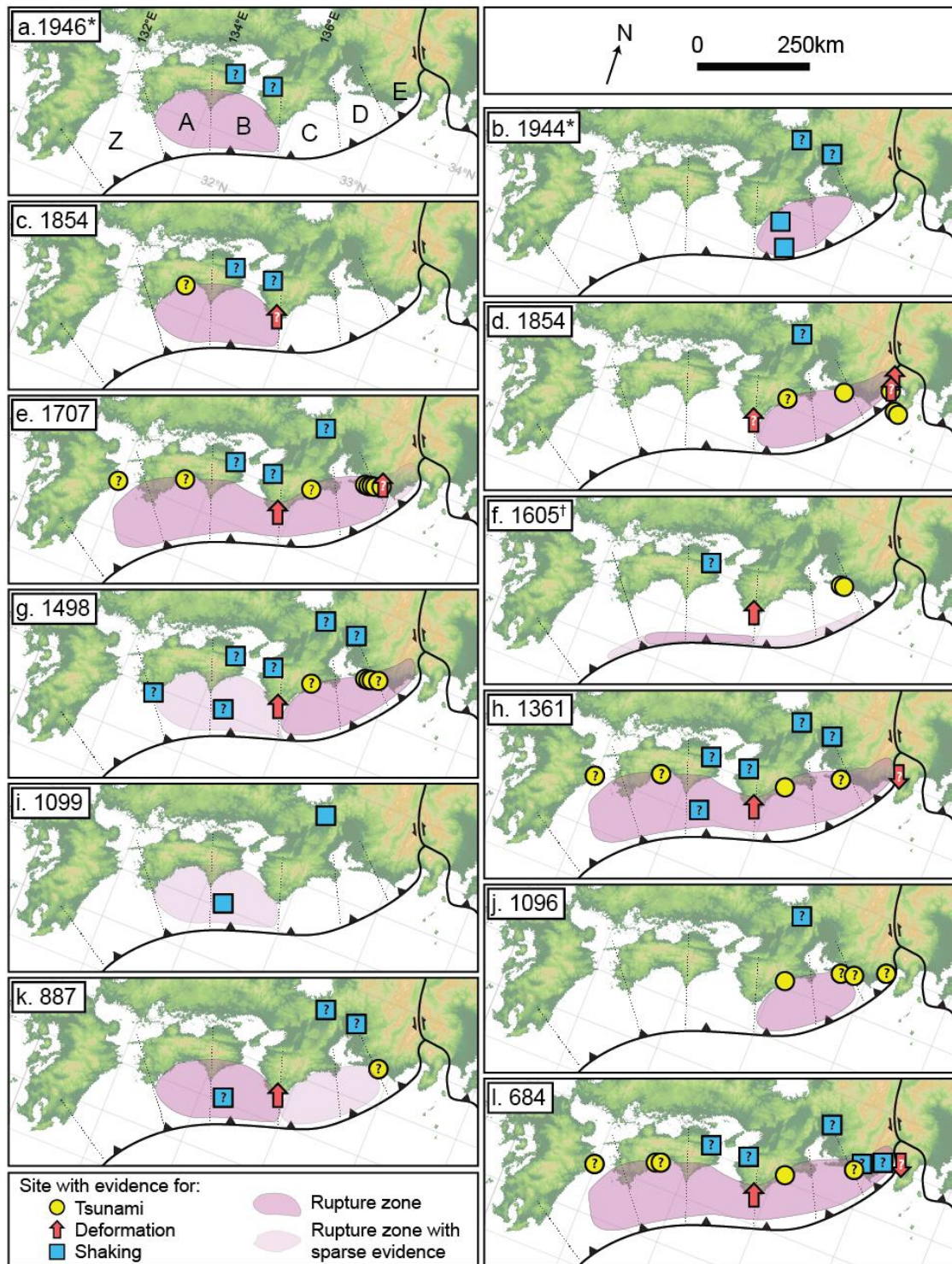
Figure 4: Summary of inferred rupture zones of historical great Nankai-Suruga Trough earthquakes and the distribution of associated geological evidence. Question marks indicate uncertainty over the chronology or the origin of evidence at a site. * Rupture zones of the AD 1946 and 1944 earthquakes are approximated from Baba and Cummins (2005) and Tanioka and Satake (2001a, b). † Rupture zone of the AD 1605 earthquake following Ando and Nakamura (2013) and Park et al. (2014).
