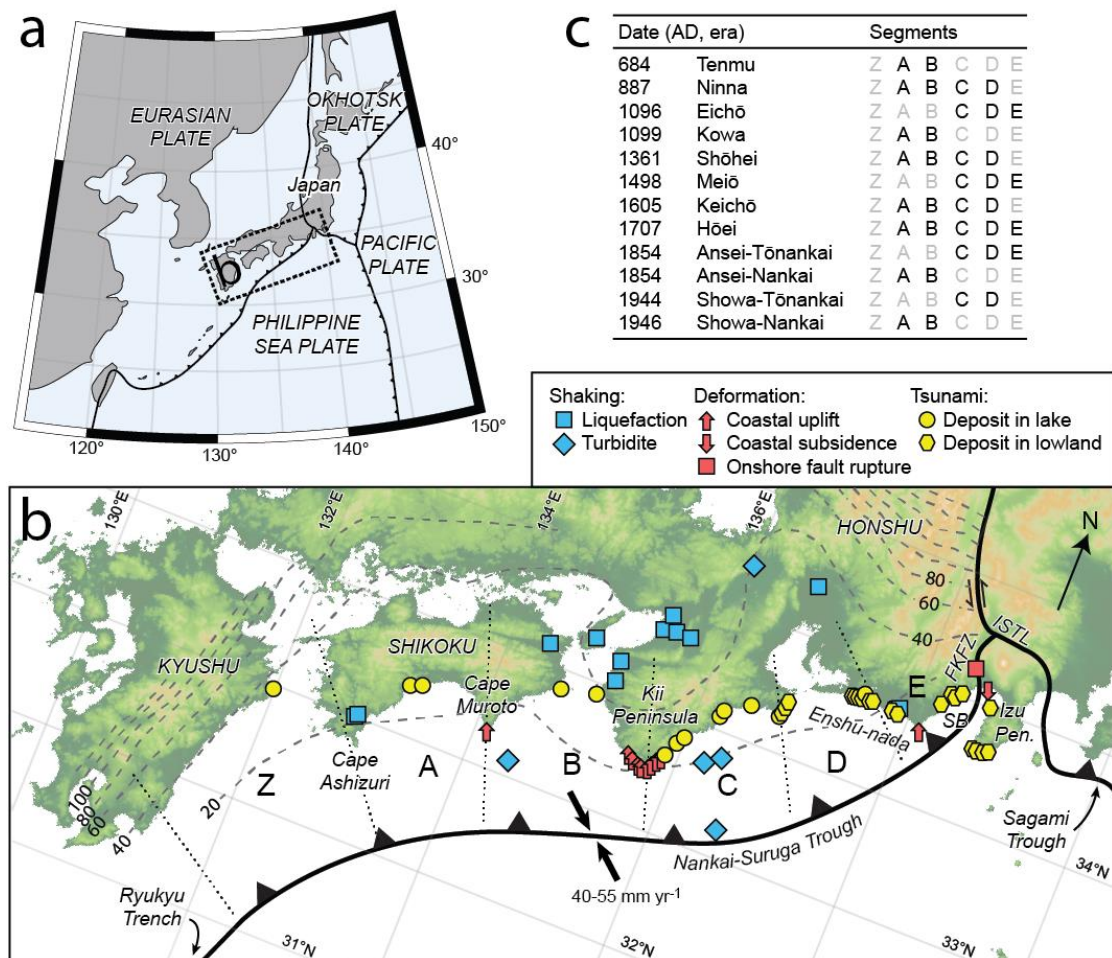
Figure 1: a) Tectonic setting of Japan, including the location of b) The Nankai-Suruga Trough, with the distribution and classification of sites discussed in this paper. Abbreviations: SB: Suruga Bay, FKFZ: Fujikawa-Kako Fault Zone, ISTL: Itoigawa-Shizuoka Tectonic Line; letters Z, A, B, C, D and E refer to seismic segments. Segment Z is also known as “Hyūga Nada”; segments A and B are collectively “Nankai”; segments C and D are collectively “Tōnankai”; segment E is “Tōkai”. Contours of the upper boundary of the subducting Philippine Sea slab marked with dashed grey lines at 20 km intervals (following Baba et al., 2002; Hirose et al., 2008; Nakajima and Hasegawa, 2007a). c) Summary of historical Nankai-Suruga Trough earthquakes, including calendar year, era name (nengō) and proposed rupture zone segments from historical records (following Ando, 1975b; Ishibashi, 2004).
