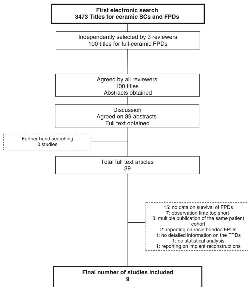
Fig. 1. Search strategy.
