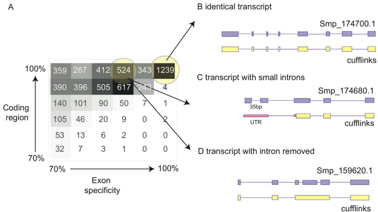
Figure 3. Improvement of gene annotation using RNA-seq. (A) Heatmap displaying comparisons between previous gene models and transcript fragments generated from Cufflinks. For each model, the extent of coding region that overlaps with a Cufflinks' model and the proportion of correctly predicted exon boundaries was calculated and categorised into bins of 70–100%. Models in this plot were excluded with less than 70% of their exon boundaries or coding regions predicted. (B), (C) and (D) Example scenarios of Cufflinks' models compared with previous gene models where (B) the Cufflinks prediction is identical to the 1,239 existing models; (C) Cufflinks fails to identify small introns; (D) Cufflinks removes incorrect introns present in the previous gene model, probably due to the improved assembly which, by correcting gaps, produced a longer single exon while the reading frame is preserved.
