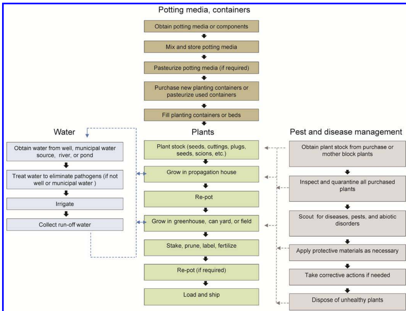
Fig. 3. An example of a simple production flow chart for a typical production container nursery. Each step in the process should be evaluated for contamination hazards by pests and pathogens.
