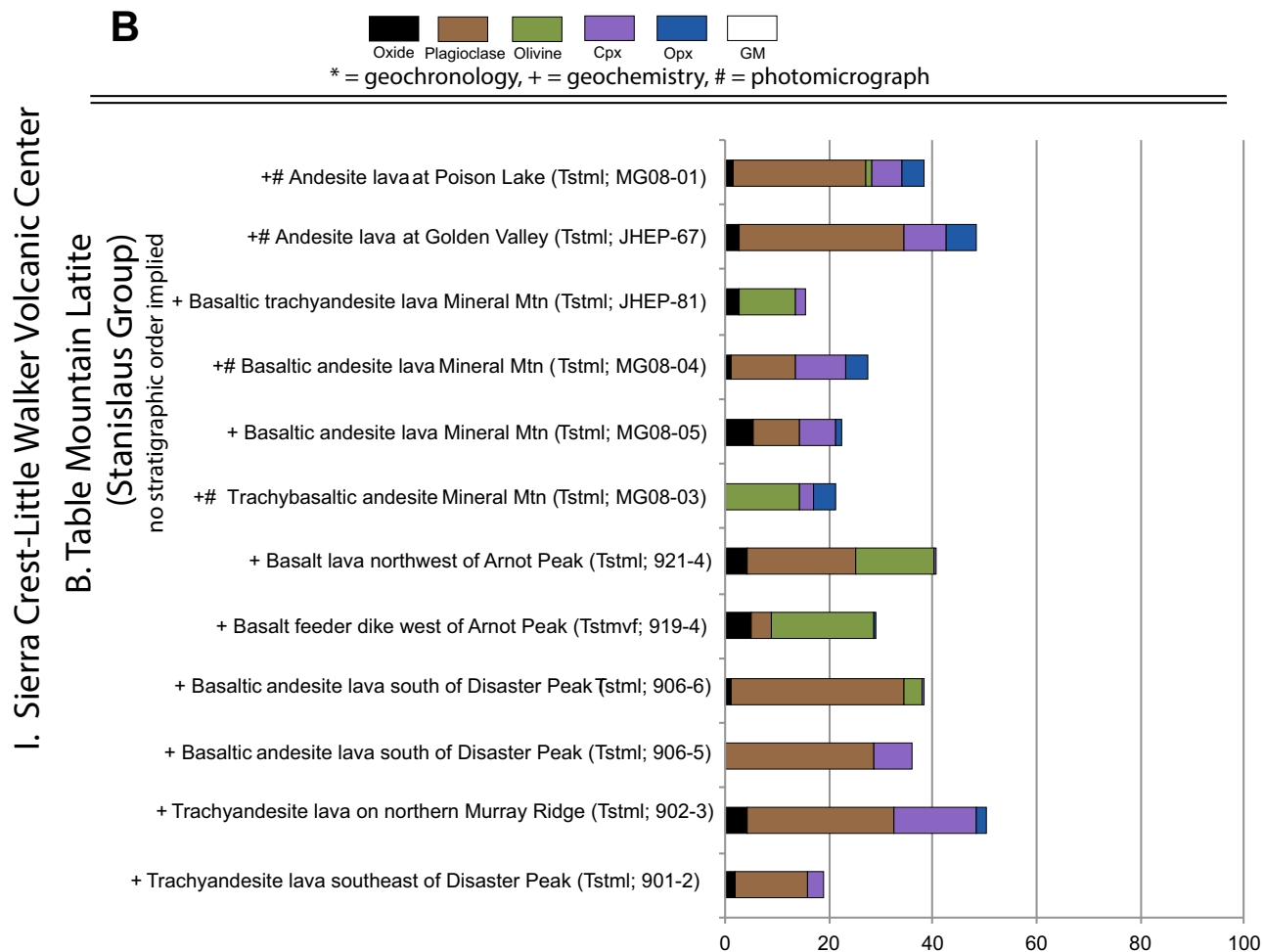
Figure 7 (continued). (B) Table Mountain Latite (Stanislaus Group).
