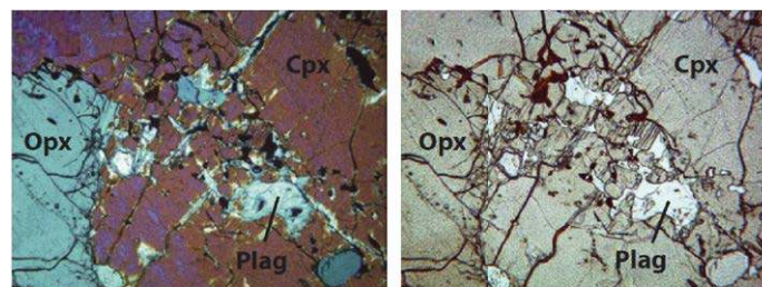
Figure 13 (continued). (D) Ebbetts Pass stratovolcano (Tdeps): Orthopyroxene (opx) olivine clinopyroxene (cpx) basaltic andesite lava (sample JHEP-9), with modal analysis (Fig. 11A) and geochemistry (Table 1) and geochronology (Fig. 5) presented here. Top pair of photos (crossed polarizers and plane light) show orthopyroxene intergrown with clinopyroxene phenocrysts with small plagioclase (Plag) inclusions. Lower photo (crossed polarizers) shows a twinned pyroxene phenocryst in a groundmass with small plagioclase crystals (Gm). (E) Ebbetts Pass stratovolcano (Tdeps): Two-pyroxene andesite lava, (sample MG-08-08), inferred to form a 25-m-thick megaslide block shed from the walls of the Ebbetts Pass pull-apart (Fig. 5), with modal analysis (Fig. 11A) and geochemistry (Table 1) and geochronology (Fig. 5) presented here. Left photo (crossed polarizers) and right photo (plane light) show 2-mm-long intergrown plagioclase phenocrysts with zoning and complex growth, and small hornblende phenocrysts. (F) Disaster Peak Formation intrusion within the altered basal fill of the Ebbetts Pass pull-apart basin (Tid, sample MG-08-10): Two-pyroxene biotite hornblende quartz (qtz) dacite intrusion. Modal analysis (Fig. 12) and geochemistry (Table 1) presented here. All photos with crossed polarizers. Top photo: Hornblende crystals with groundmass cores; also, twinned pyroxene; microcrystalline groundmass. Middle photo: embayed or xenocrystic quartz and small intergrown hornblende crystals. Lower photo: Biotite intergrown with partially rimmed plagioclase; hornblende crystals with groundmass cores; and small pyroxenes.
