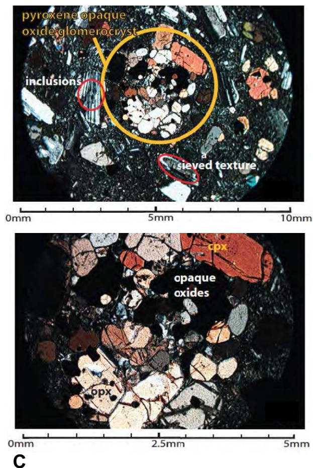
Figure 9 (continued). (C) Table Mountain Latite (Tstml), Stanislaus Group: Two-pyroxene olivine andesite lava (sample MG08-01), with modal analysis (Fig. 7B) and whole-rock geochemistry (Table 1) presented here. Top photo (crossed polarizers) shows glomerocryst of pyroxene and opaque oxides, as well as sieve-textured plagioclase, and plagioclase with inclusions. Bottom photo (crossed polarizers) is magnified view of two-pyroxene and opaque oxide glomerocryst, showing subrounded crystals 0.25 mm to 1.5 mm in length (cpx—clinopyroxene; opx—orthopyroxene). (D) Table Mountain Latite (Tstml), Stanislaus Group: Two-pyroxene basaltic andesite lava (sample MG08-04), with modal analysis (Fig. 7B) and whole-rock geochemistry (Table 1) presented here. Top photo (plane-polarized light) shows larger (6-mm-long) plagioclase phenocrysts with sieve textures near the rim, and clear euhedral plagioclase on the rim, with smaller phenocrysts (1–2 mm) showing sieve-textured cores and clear rims. This may indicate that there was a reaction between the crystals and one magma, followed by renewed growth in a magma of different composition. Lower photo (crossed polarizers) shows twinned and untwinned clinopyroxene.
