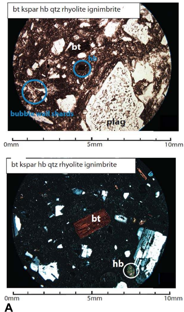
Figure 13 (on this and following two pages). Photomicrographs from the Ebbetts Pass volcanic center and pull-apart basin (samples plotted on Fig. 2B): (A) Lower silicic section: Biotite (bt) sanidine hornblende (hb) quartz (qtz) rhyolite welded ignimbrite (Tdpwi; Fig. 2B), sample MG08-07, with modal analysis (Fig. 11A) and whole-rock geochemistry (Table 1) and geochronology (Fig. 5) presented herein. Kspar—K-feldspar. This sample comes from a less strongly welded part of the overall very strongly welded ignimbrite, and so in plane-polarized light (upper photo), bubble-wall shards are obvious. Biotite (bt) and hornblende (hb), as well as glass matrix, are shown in crossed polarizers (lower photo). (B) Lower silicic section: Hornblende biotite rhyolite lava (Tdplr, sample JHEP-43), with modal analysis (Fig. 11A) and whole-rock geochemistry (Table 1) presented herein. Left photo (crossed polarizers) shows biotite and plagioclase in a glass groundmass. In plane light (right photo), the glass groundmass is clear and hard to distinguish from plagioclase, which is relatively free of inclusions. (C) Lower silicic section (Fig. 5): Hornblende biotite sanidine quartz silicic lava (Tdplr, sample JHEP-53), with modal analysis presented herein (Fig. 11A). Left photo (crossed polarizers) shows biotite and plagioclase enclosed by a hornblende phenocryst, with zoned plagioclase phenocrysts in a fine-grained felsitic groundmass. In plane light (right photo), the biotite crystals are barely visible within the hornblende phenocryst.
