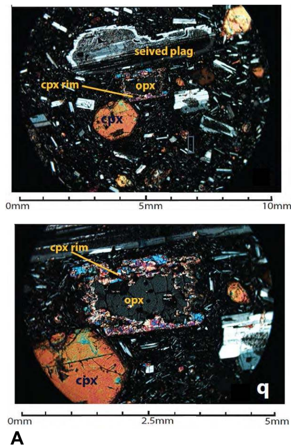
Figure 9 (on this and following four pages). Photomicrographs from the Sierra Crest graben-vent system (samples plotted on Fig. 2B): (A) Relief Peak Formation lava (Trpl): Two-pyroxene (pyx) basaltic andesite lava mantled with flow breccia, sample MG08-02, with modal analysis (Fig. 7A) and whole-rock geochemistry (Table 1) presented here; crossed polarizers. Top photo shows two pyroxenes and plagioclase in a glassy groundmass, and a 6-mm-long, sieve-textured, embayed, rimmed plagioclase feldspar. Lower photo shows an orthopyroxene crystal rimmed by a 0.5-mm-thick layer of clinopyroxene, adjacent to a large (2 mm) euhedral clinopyroxene crystal. (B) Table Mountain Latite (Tstml), Stanislaus Group: Two-pyroxene andesite lava (sample JHEP-67) with modal analysis (Fig. 7B) and whole-rock geochemistry (Table 1) presented here. Top photos (crossed polarizers and plane-polarized light) show sieve-textured plagioclase common to Table Mountain Latite. Bottom photos (crossed polarizers and plane-polarized light) show twinned phenocrysts of clinopyroxene.
