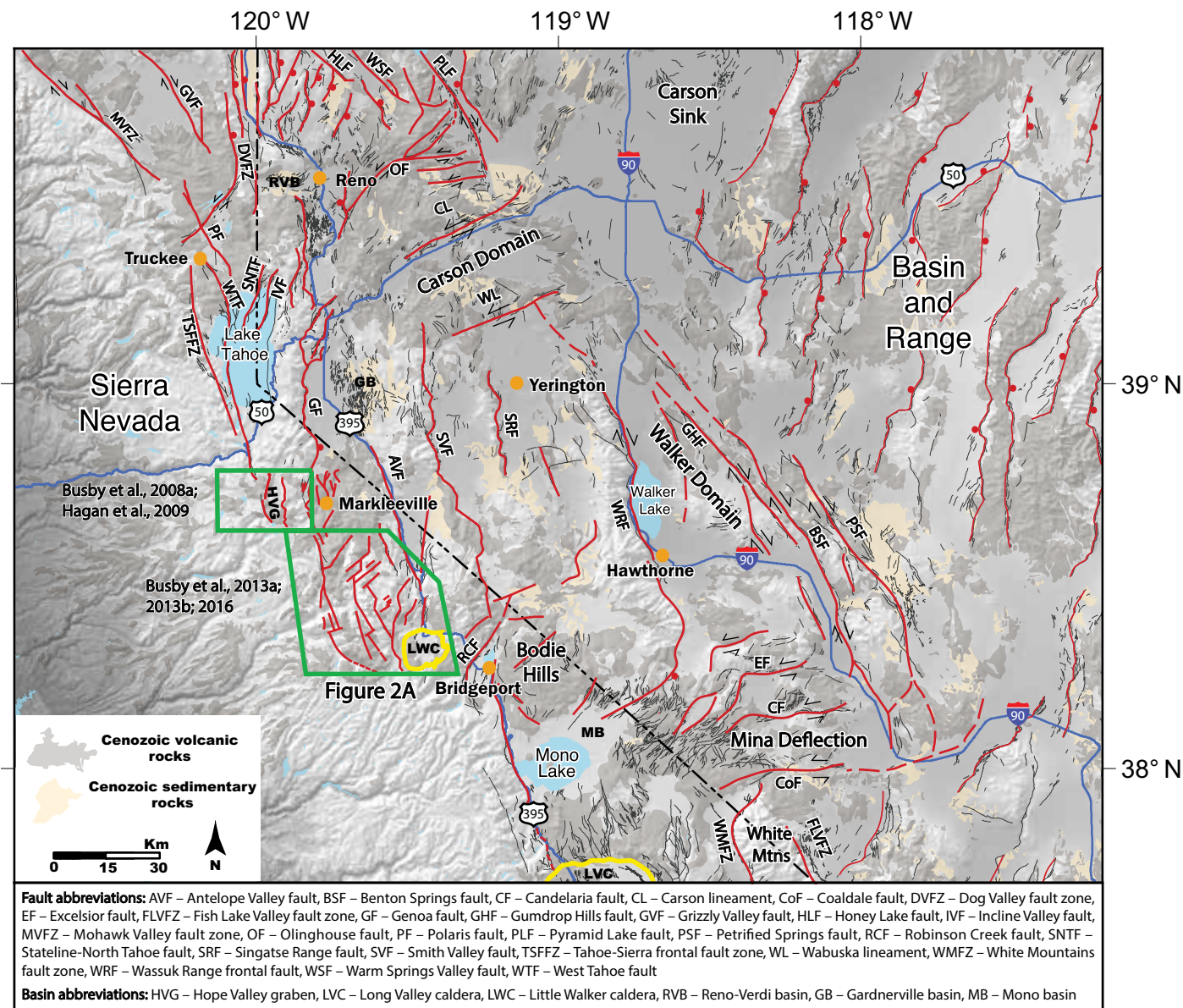
Figure 1. Central Walker Lane and adjacent areas, showing Cenozoic volcanic and sedimentary rocks and faults, modified from Faulds and Henry (2008), Wesnousky et al. (2012), and Bormann et al. (2016). Additional map data are from Kent et al. (2005), Crafford (2007), Hunter et al. (2011), Cashman et al. (2009, 2012), Jayko and Bursik (2012), John et al. (2012), Carlson et al. (2013), Nagorsen-Rinke et al. (2013), Carlson and Faulds (2014), and John et al. (2015a, 2015b). This is the first published Walker Lane compilation map to show faults of the Walker Lane pull-apart basins described in this paper, outlined in the box labeled Fig. 2A (Busby et al., 2013a, 2013b, 2016). Our compilation map also includes our Walker Lane faults mapped to the north at Carson Pass (Hagan et al., 2009), shown on Figure 4.
