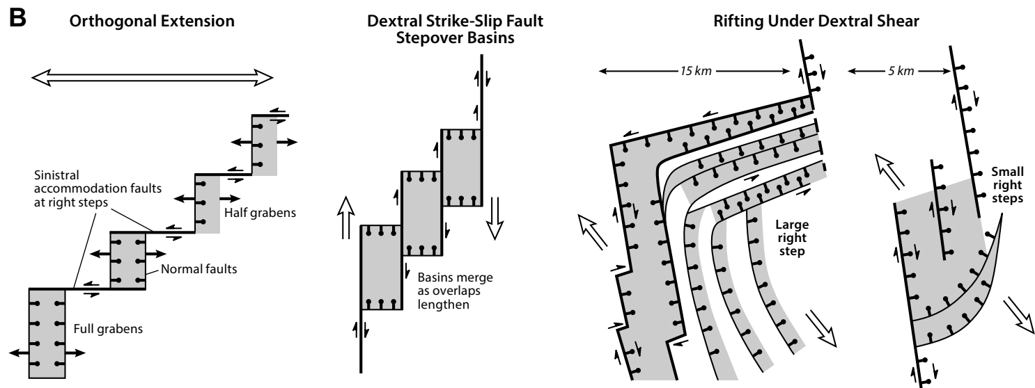
Figure 4 (continued). (B) Simplified depiction of faults and basins formed under orthogonal extension (panel one) and under right-stepping dextral strike-slip faults (panel two), for comparison with faults and basins formed under transension/rifting under dextral shear. Rifting under dextral shear is illustrated for the transtensional faults and basins of the Sierra Crest–Little Walker pull-apart (panel three), and the Ebbetts Pass pull-apart (panel four). In both, obliquity between Sierra Nevada and North American microplate motion (large open arrows) and the orientation of faults resulted in approximately N-S normal-dextral faults. A large right step was accommodated by a system of approximately NE normal-sinistral faults in the Sierra Crest–Little Walker pull-apart basin (panel three). In contrast, in the Ebbetts Pass pull-apart basin, series of small right steps along approximately N-S normal-dextral faults produced a smaller pull-apart structure, with normal faults along its trailing edge (panel four).
