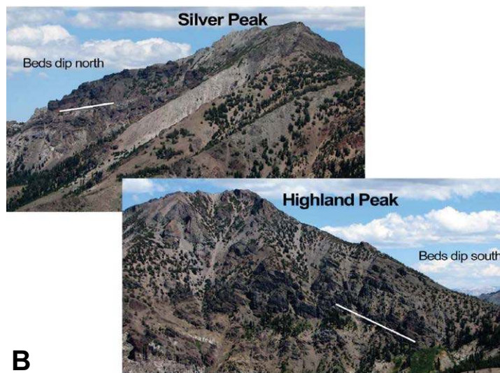
Figure 10 (on this and following three pages). Outcrop photos from the Ebbetts Pass volcanic center; see stratigraphy in Figures 2 and 5. (A) Oblique aerial photo of Ebbetts Pass stratovolcano (Tdeps); top partially eroded. (B) View of Ebbetts Pass stratovolcano, looking eastward from the Sierra Crest on the footwall of the Noble Canyon fault (Tdeps; Fig. 2), showing northward primary dips on the north flank of the edifice (north of Silver Peak) and southward dips on the south flank of the edifice (south of Highland Peak; see Fig. 2B). Silver Peak and Highland Peak are formed of silicic intrusions at the eroded crest of the stratovolcano. (C) Basal section of black olivine two-pyroxene basaltic andesite lavas of the Ebbetts Pass stratovolcano on the footwall of the Noble Canyon fault, along the Sierra Crest ~1.5 km south of Ebbetts Pass. Photo shows primary westward dips away from the center of the stratovolcano. See sample JHEP-9 for geochronology, geochemistry, photomicrograph, and modal analysis. At this locality, the basal basaltic andesite lava section has an underlying white clinopyroxene-orthopyroxene quartz lava (sample JHEP-10; Fig. 11A) that is flow banded, with a flow-top breccia (see text for discussion).
