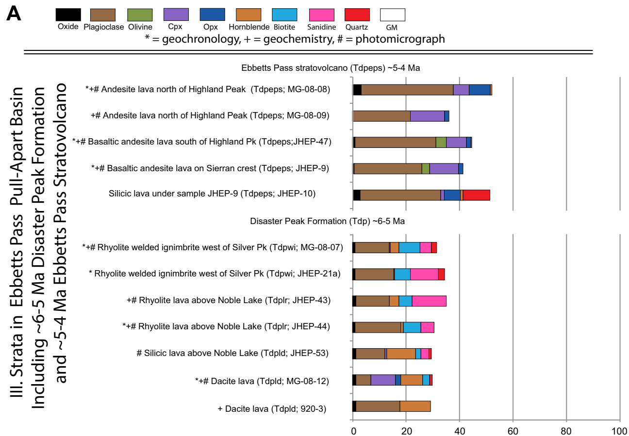
Figure 11 (on this and following page). Modal analysis of strata in the Ebbetts Pass volcanic center and pull-apart basin. (A) Strata within the pull-apart basin divided into time frames: Disaster Peak Formation (ca. 6–5 Ma), also referred to here as the lower silicic section (Fig. 4); and Ebbetts Pass stratovolcano (ca. 5–4 Ma). (B) Lavas along the east margin of the Ebbetts Pass pull-apart basin (east of the Wolf Creek fault; Fig. 2B), tentatively inferred to have erupted from the Ebbetts Pass stratovolcano. Cpx—clinopyroxene, Opx—orthopyroxene, GM—groundmass.
