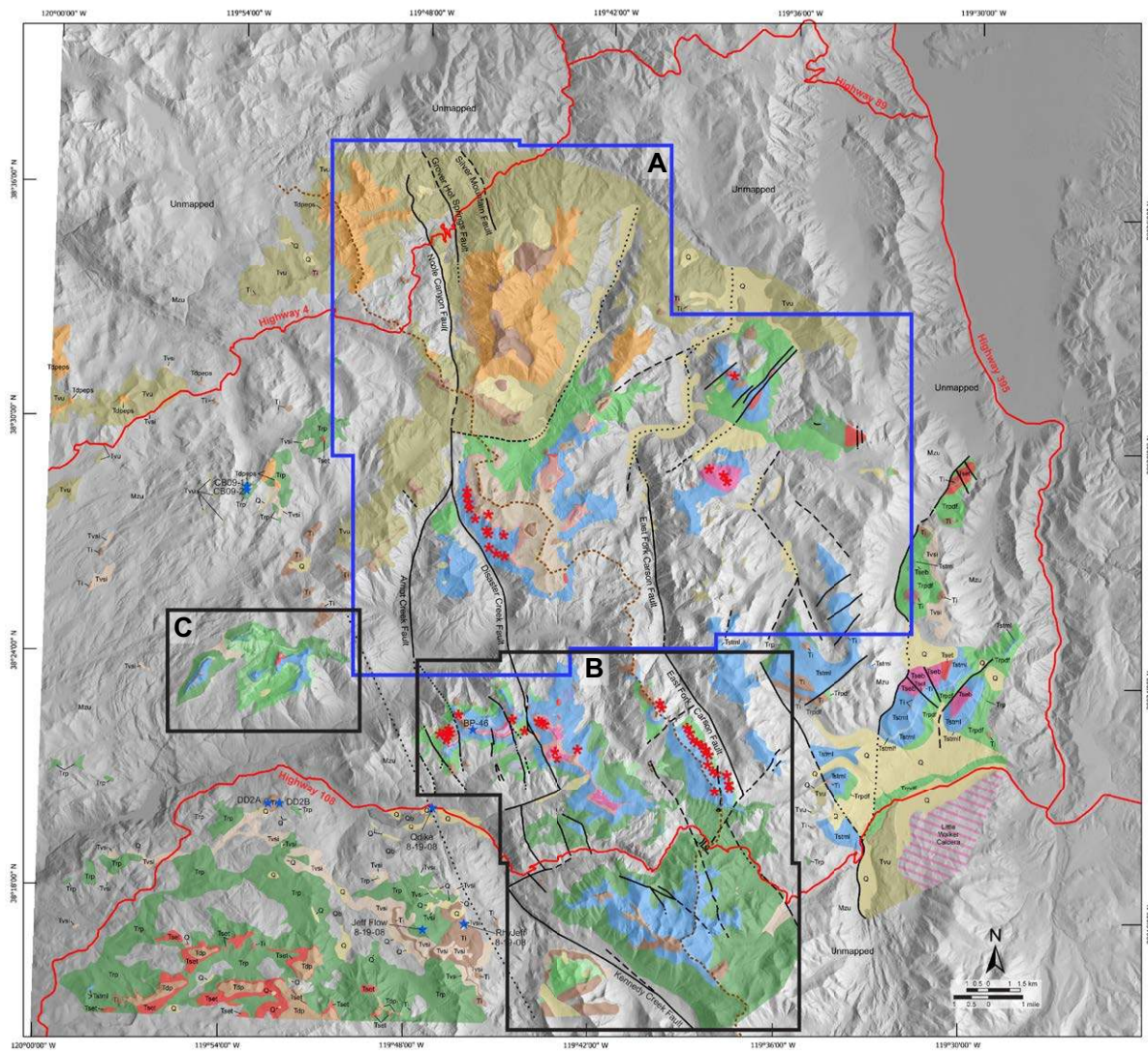
Figure 2 (on this and following page). (A) Generalized geologic map of Tertiary rocks of the Sonora Pass to Ebbetts Pass area, central Sierra Nevada, from Busby et al. (2016). Location is on Figure 1. All mapping was done by Busby and her graduate students (Jeanette Hagan, Alice Koerner, Ben Melosh, Dylan Rood) and her postdoctoral researcher (Graham Andrews) between 2001 and 2012, drawing on previous work by Slemmons (1953), an unpublished 1979 map provided to Busby by Slemmons, Keith et al. (1982), Huber (1983a, 1983b), Armin et al. (1984), and Roelofs (2004). Insets on upper right show location and previous mapping. Red stars highlight vents for Stanislaus Group volcanic rocks. Map unit contacts and labels are not drawn in this generalized map because it is so reduced; instead, a detailed map of area A is shown in Figure 2B, and detailed maps of areas B and C were published in Busby et al. (2016). Some samples discussed in this paper lie outside the area of Map A and are plotted here. To view the full-sized version of this map, please visit https://doi.org/10.1130/GES01398.m1 or the full-text article on www.gsapubs.org .
