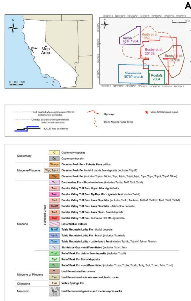
Figure 2 (on this and following page). (A) Generalized geologic map of Tertiary rocks of the Sonora Pass to Ebbetts Pass area, central Sierra Nevada, from Busby et al. (2016). Location is on Figure 1. All mapping was done by Busby and her graduate students (Jeanette Hagan, Alice Koerner, Ben Melosh, Dylan Rood) and her postdoctoral researcher (Graham Andrews) between 2001 and 2012, drawing on previous work by Slemmons (1953), an unpublished 1979 map provided to Busby by Slemmons, Keith et al. (1982), Huber (1983a, 1983b), Armin et al. (1984), and Roelofs (2004). Insets on upper right show location and previous mapping. Red stars highlight vents for Stanislaus Group volcanic rocks. Map unit contacts and labels are not drawn in this generalized map because it is so reduced; instead, a detailed map of area A is shown in Figure 2B, and detailed maps of areas B and C were published in Busby et al. (2016). Some samples discussed in this paper lie outside the area of Map A and are plotted here. To view the full-sized version of this map, please visit https://doi.org/10.1130/GES01398.m1 or the full-text article on www.gsapubs.org .
