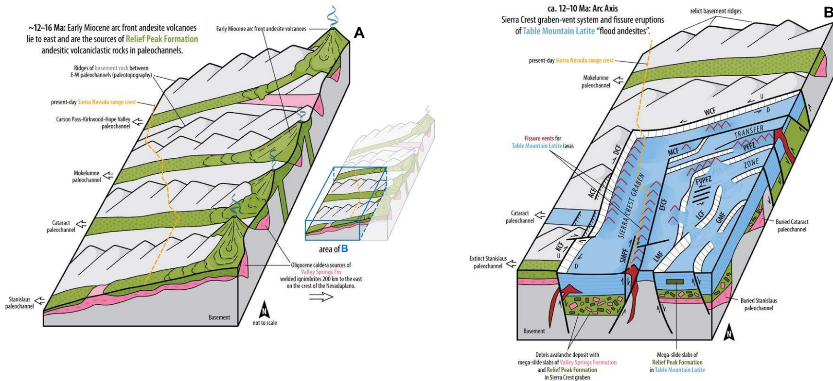
Figure 14 (on this and following two pages). Block diagrams illustrating the tectonic and magmatic evolution of the Sierra Crest–Little Walker volcanic center and pull-apart basin, and the Ebbetts Pass volcanic center and pull-apart basin. Data to support these interpretations are given in Figures 2 through 13, and Table 1, and the text. Faults are labeled to facilitate comparison to Figures 2 and 4: ACF—Arnot Creek fault, CLF—Chango Lake fault, DCF—Disaster Creek fault, EFCF—East Fork Carson fault, FVPFZ—Fish Valley Peak fault zone, GHSF—Grover Hot Springs fault, GMF—Grouse Meadows fault, KCF—Kennedy Creek fault, LCF—Lost Cannon fault, LMF—Leavitt Meadow fault, LWC—Little Walker caldera, MCF—Murray Canyon fault, NCF—Noble Canyon fault, PPFZ—Poison Flat fault zone, SMPF—St. Mary’s Pass fault, WCF—Wolf Creek fault. Abbreviations for formations: EVT—Eureka Valley Tuff, DP—Disaster Peak Formation, R Pk—Relief Peak Formation, TML—Table Mountain Latite, VS Fm—Valley Springs Formation. (A) Main paleogeographic elements immediately prior to the onset of Walker Lane transtension (ca. 16–12 Ma), with the present-day position of Sierra Nevada range crest given for reference (also see Figs. 2A, 4). By ca. 16–12 Ma, the arc front had swept westward across Nevada into the westernmost Nevada region (see Busby and Putirka, 2009; Busby, 2012, 2013). The volcanoes lay just to the east of the study area and shed andesitic volcanoclastic debris into the Stanislaus, Cataract, and Mokelumne paleochannels, mapped as Relief Peak Formation. Similar age-equivalent deposits also occur in the Carson Pass–Kirkwood paleochannel to the north, described by Busby et al. (2008a) and Hagan et al. (2009). Paleorelief and axial gradients were high, with the “paleochannels” actually consisting of rugged canyons with abundant fluvial boulders. The basal fill of the paleochannels consists of Oligocene Valley Springs Formation welded ignimbrites resting on Mesozoic basement along unconformity 1 (Fig. 3). The unconformity at the base of Relief Springs Formation (unconformity 2; Fig. 3) commonly downcuts through Valley Springs Formation to merge with unconformity 1, where Relief Peak Formation paleochannel fill rests directly on Mesozoic basement. Relief Peak Formation paleochannel fill consists of stratified andesitic debris flow and fluvial deposits, representing down-paleochannel reworking of eruptive products, as well as andesitic block-and-ash-flow tuffs, generated by lava dome collapse. Lavas only occur at one locality (The Dardanelles; Busby et al., 2016), and these are basalt, which can flow tens of kilometers from the vent. Inset block diagram shows the area of part B. (B) By 12 Ma, the arc front had swept westward into what is now the Sierra Nevada, and a very large Walker Lane pull-apart basin began to form in the arc axis, referred to as the Sierra Crest–Little Walker pull-apart and volcanic center. The onset of transtensional faulting was marked by deposition of mass-transport deposits in the grabens, consisting of massive debris-flow deposits and debris-avalanche deposits with megaslide blocks of Relief Peak Formation and Valley Springs Formation. Relief Peak Formation and Valley Springs Formation strata were stripped off adjacent horst blocks; for example, see Table Mountain Latite resting directly on basement in the horst block on the front of the block diagram, with older units in the grabens on either side. Mass wasting began by 12.2 \pm 0.1 Ma, as shown by the age of an andesite sill intruding mass-transport deposits, and persisted until 10.39 \pm 0.18 Ma, as shown by a date on a block-and-ash-flow tuff within a megaslide block beneath Table Mountain Latite. Transtension then triggered eruption of high-K volcanic rocks of the Stanislaus Group, including Table Mountain Latite (this time frame) and lavas and ignimbrites of the Eureka Valley Tuff (next time frame; see part C), by allowing parental magmas with lower degrees of partial melting to ascend (Putirka and Busby, 2007; Putirka et al., 2012). The Table Mountain Latite includes basalt, trachybasaltic andesite, and trachyandesite, and lesser basaltic andesite and andesite lavas erupted from fault-controlled fissures (red inverted V’s). The graben-filling Table Mountain Latite (TML) lavas were ponded to thicknesses of up to 400 m. The N–S normal faults (see U and D symbols) are dextral oblique (see arrows), and the NE normal faults are sinistral oblique, consistent with the overall geometry of the fault system, which is a releasing right step (Fig. 4B; Busby et al., 2013a). “Tectonostratigraphic recycling” continued, with avalanching of Relief Peak Formation megaslide slabs into grabens while they filled with Table Mountain Latite lavas (Fig. 5). Paleochannels were largely destroyed by faulting and avalanching within the pull-apart structure. Buried Stanislaus and Cataract paleochannels are depicted along the east side of the pull-apart basin, where they are preserved on the hanging wall of the Lost Cannon fault and the southernmost East Fork Carson fault (Fig. 2A). There, Valley Springs Formation is overlain by Relief Peak Formation mass-transport deposits, with abundant megaslide slabs of Valley Springs Formation. Along the western margin of the pull-apart basin, the Stanislaus paleochannel was beheaded by faulting (“extinct Stanislaus paleochannel”). Growth faults formed in the Cataract paleochannel but did not dismember it. The Mokelumne paleochannel to the north remained unfaulted.
