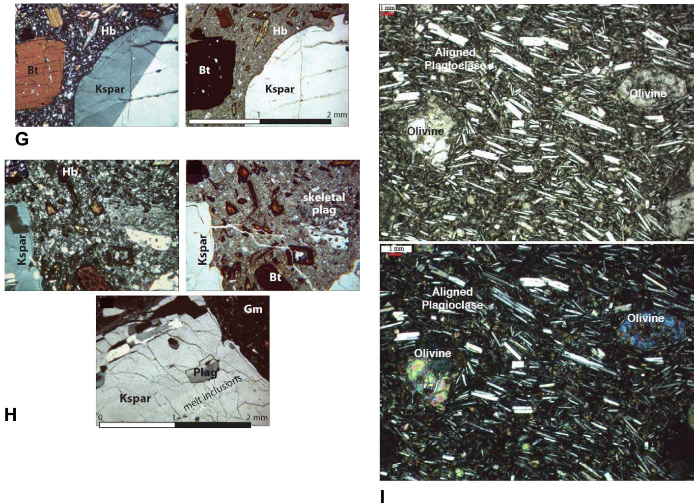
Figure 13 (continued). (G) Ebbetts Pass stratovolcano: Hornblende biotite quartz dacite intrusion of Highland Peak (Tdpid, sample JHEP-49), with geochronology (Fig. 5), whole-rock geochemistry (Table 1), and modal analysis (Fig. 12) presented here, in crossed polarizers (left) and plane-polarized light (right). Biotite (Bt) is up to 1 mm long, with smaller hornblende (Hb), and twinned feldspar (Kspar). (H) Ebbetts Pass stratovolcano: Dacite intrusion of Highland Peak (Tdpid, sample JHEP-50), with geochemistry presented here (Table 1). Upper-left photo (crossed polarizers) and upper-right photo (plane light) show potassium feldspar (sanidine), skeletal plagioclase, and biotite phenocrysts. Lower photo (crossed polarizers) shows plagioclase crystals enclosed by >2-mm-long sanidine crystal with melt inclusions. (I) Postsubduction rift basaltic andesite (Fig. 5): Olivine two-pyroxene basaltic andesite intrusion (sample 901-3, same body as JHEP-54; whole-rock geochemistry in Table 1). The olivine is fresh, suggesting this is related to the young ( 3.65 \pm 0.03 Ma plag) postsubduction rift basalt at Disaster Peak. Although age controls on this intrusion are poor because it cuts granitic basement (Fig. 5B) and is undated, we suspect that all of the olivine basalt plugs shown on Figures 2A and 2B are younger than 4 Ma in age. Top image is plane-polarized light, and bottom image is crossed polarized light.
