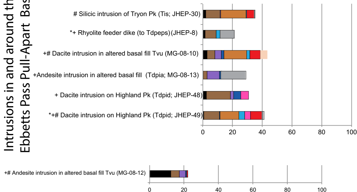
Figure 12. Modal analysis of intrusions in and around the Ebbetts Pass volcanic center and pull-apart basin. Cpx—clinopyroxene, Opx—orthopyroxene, GM—groundmass.
