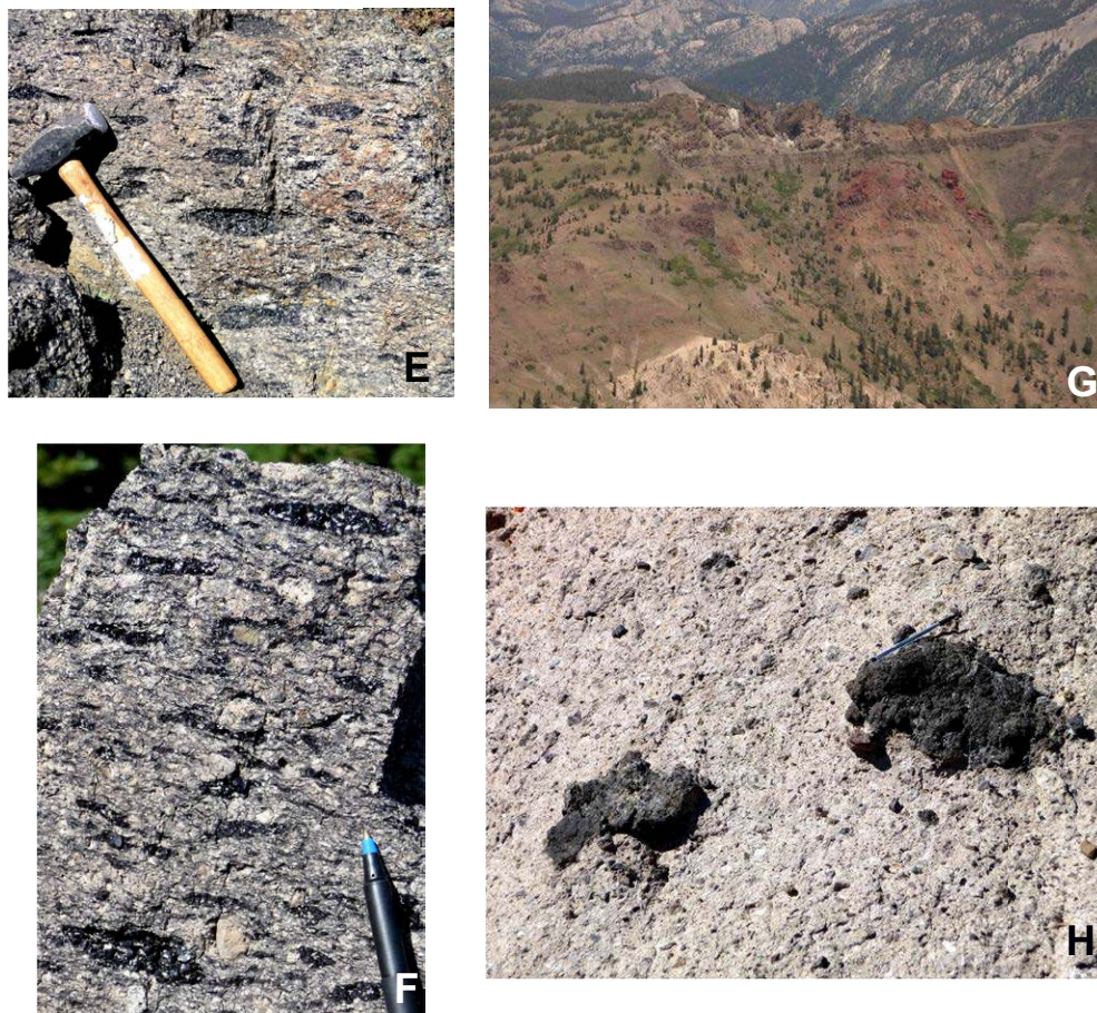
Figure 6 ( continued ). (E) Eureka Valley Tuff, Tollhouse Flat Member, showing trachydacite welded ignimbrite with large black glassy fiamme and small white/light-gray silicic volcanic rock fragments. (F) Close-up of Eureka Valley Tuff, Tollhouse Flat Member, showing light-gray volcanic rock fragments common to all ignimbrite members of the Eureka Valley Tuff (Fig. 7C). (G) Cliff-face cross section through a cinder cone (red), in the Lava Flow Member of the Eureka Valley Tuff. This basalt cinder cone is cut by an olivine basalt feeder dike that vented olivine basalt lava flows within the Lava Flow Member of the Eureka Valley Tuff. Depositionally above the red cinder cone rocks, forming an ~10-m-thick black horizontal band, is the basal vitrophyre of the By Day Member of the Eureka Valley Tuff. This in turn is overlain by a debris-avalanche deposit shed from a graben-bounding fault during accumulation of the Stanislaus Group: Note white blocks of Upper Member Eureka Valley Tuff, including one with bedding standing on end. (H) Nonwelded upper part of the By Day Member of the Eureka Valley Tuff, showing uncompacted black pumice blocks and lapilli. Small white clasts are volcanic rock fragments common to all ignimbrites of the Eureka Valley Tuff (Fig. 7C); for photomicrograph with volcanic rock fragments, see Figure 9I. Pen for scale (resting on pumice block).
