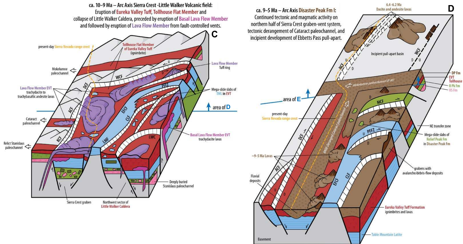
Figure 14 (continued). (C) Transtension and volcanism continued in the arc axis, resulting in formation of the Little Walker caldera, which erupted three trachydacite ignimbrites, while lavas continued to erupt across the Sierra Crest–Little Walker volcanic center, evolving to include trachydacites. This time frame shows the period after eruption of Basal Lava Flow Member and Tollhouse Flat Member (Fig. 5), during eruption of the Lava Flow Member. The NW sector of the Little Walker caldera is shown in the bottom-right corner, which formed in the area of maximum transtension. The thickness of the caldera fill is not known (Priest, 1979), nor is it known if it contains slide blocks; it is heavily altered and intruded (Busby’s field observations). Due to the great mobility of pyroclastic flows, the Tollhouse Flat Member of the Eureka Valley Tuff (EVT) was deposited in all grabens and paleochannels, including the relict Stanislaus paleochannel, as well as the Mokelumne paleochannel, which has no other Stanislaus Group units. The entire Sierra Crest–Little Walker volcanic center began erupting trachydacite lavas, in addition to continued eruption of basalt to trachyandesite lavas, prior to and after eruption of the Tollhouse Flat Member welded ignimbrite from the caldera. These are shown as Basal Lava Flow Member and Lava Flow Member of the Eureka Valley Tuff (Fig. 5). Lavas of the Eureka Valley Tuff were all erupted from fault-controlled vents, except for those associated with the caldera described by Priest (1979). Widespread eruption of the Lava Flow Member (shown here) was followed by eruptions of the By Day Member welded ignimbrite and Upper Member nonwelded ignimbrite from the Little Walker caldera (not shown here). The last stage of high- K_2O magmatism is recorded by a single black shoshonite lava up to 60 m thick (Dardanelles Formation, not shown), which erupted from a vent along the west side of the Sierra Crest graben and flowed down the Cataract paleochannel. “Tectono-stratigraphic recycling” continued throughout eruption of the Stanislaus Group. After eruption of the Stanislaus Group, volcanism and faulting ended in the southern half of the Sierra Crest–Little Walker volcanic center, so the next time frame shows only the northern half (part D). (D) This time frame shows andesitic magmatism and ongoing subsidence in the northern part of the Sierra Crest–Little Walker volcanic center and pull-apart basin, after high- K_2O magmatism ended (the southern half became inactive; see text). For simplicity, all of the members of the underlying Eureka Valley Tuff are generalized into one unit. During this time frame, the Cataract paleochannel (shown in A–C), became deranged from its earlier E–W (Nevadaplano) trend into the approximately N–S Walker Lane Basin trend shown here (described in detail by Busby et al., 2016). We infer that it fed into the Mokelumne paleochannel until that paleochannel got beheaded, as shown in the next time slice (part E). Catastrophic sedimentation continued in the NE transfer zone basins with massive debris-flow deposits. Basalt, basaltic andesite, and andesite lavas erupted from fault-controlled vents with vent facies deposits, and lava domes collapsed to produce block-and-ash-flow tuffs of basaltic andesite to andesite/dacite compositions. Most intrusions are sited along faults. Tectono-stratigraphic recycling continued, as megaslide slabs of older volcanic units were shed into grabens filling with Disaster Peak Formation. Incipient development of the Ebbetts Pass pull-apart basin and volcanic center began in this time frame, with eruption of 6.4–6.2 Ma dacite and andesite lavas from the Noble Canyon fault, shown as relict lavas and megaslide blocks in part E. However, subsidence and volcanism had not yet disrupted the Mokelumne paleochannel in this time frame (Busby et al., 2016). By 5 Ma, the northern part of the Sierra Crest–Little Walker volcanic center and pull-apart became inactive, so the next time frame (part E) shows only the Ebbetts Pass volcanic center and pull-apart.
