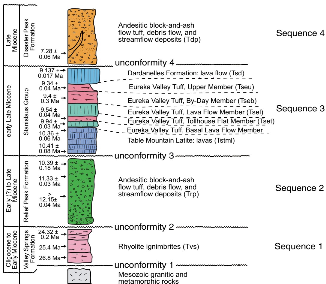
Figure 3. Generalized stratigraphy of Cenozoic paleochannel fill in the Sonora Pass region, central Sierra Nevada, California, modified from Busby et al. (2013a). Thicknesses of units are variable and not shown to scale. Mappable erosional unconformities divide the section into four sequences that have been correlated with unconformities in other central Sierra Nevada paleochannels (Busby et al., 2008a, 2008b; Busby and Putirka, 2009; Busby, 2012). Ages are from Busby et al. (2008b), Busby and Putirka (2009), Busby et al. (2013b), and this paper (Fig. 5). The two older ages on the Valley Springs Formation are based on correlations made by Chris Henry (2013, written commun.).
