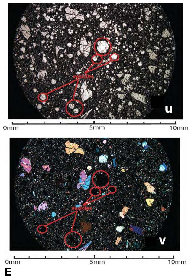
Figure 9 (continued). (E) Table Mountain Latite (Tstml), Stanislaus Group: Olivine (ol) two-pyroxene trachybasaltic andesite lava (sample MG08-03), with modal analysis (Fig. 7B) and whole-rock geochemistry (Table 1) presented here. Top photo is plane-polarized light, and lower photo is crossed polarizers. This sample is unusual for lacking plagioclase phenocrysts. It has small phenocrysts of olivine in addition to the larger pyroxene crystals. Vesicles are filled with chlorite. (F) Basal Lava Flow Member of the Eureka Valley Tuff (Tselbt), Stanislaus Group: Two-pyroxene hornblende biotite trachydacite intrusion that cuts Table Mountain Latite and passes upward into a lava flow that overlies Table Mountain Latite (Tselbt, sample JHEP-88), dated at 9.84 \pm 0.03 Ma (Fig. 4), with modal analysis (Fig. 7B) and whole-rock geochemistry (Table 1) presented here. Top photos (crossed polarizers and plane-polarized light) show sieve-textured plagioclase phenocrysts, typical of Stanislaus Group, in a fine-grained to glassy groundmass. Bottom-left photo (crossed polarizers) shows biotite, pyroxene, and sieve-textured plagioclase (plag) crystals. Bottom-right photo (plane-polarized light) shows biotite (Bt), hornblende (Hb), pyroxene, and plagioclase phenocrysts.
