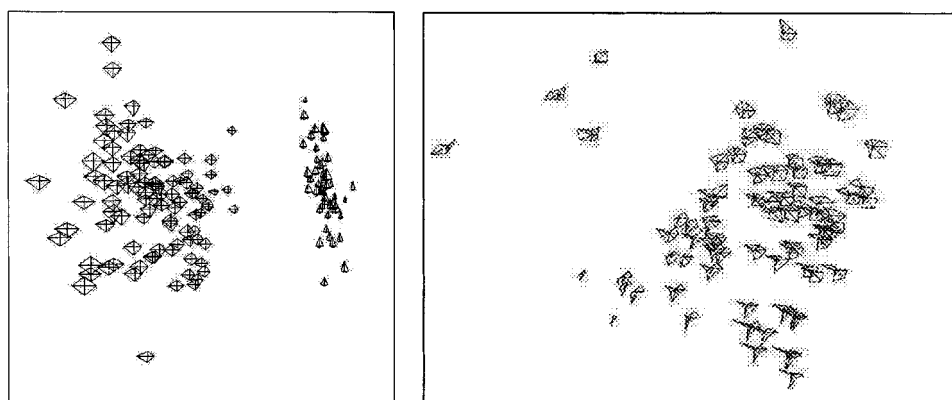
Figure 4 Star glyphs of the Iris and cars data sets with position based on the first two principal components.
