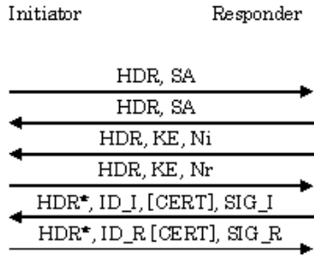
Figure 1: IPsec Main Mode
