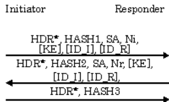
Figure 3: IPsec Quick Mode
