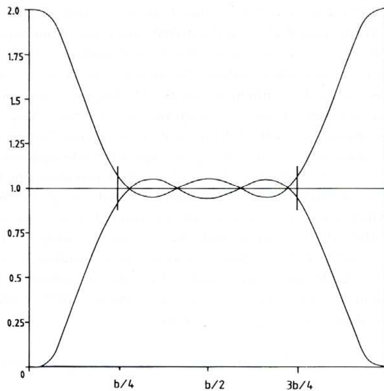
Fig. 4. Variation of spectral density across the basin.
