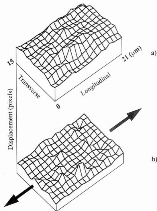
FIG. 6. A 3-D view of the u - and v -microextensometry displacement components. a) shows the u -component vector of (transverse) fiber displacement; b) displays the longitudinal displacement component coincident to the direction of applied strain (fiber longitudinal axis). Kraft pulped black spruce 47% yield. The arrows represent the direction of applied displacement. Displacement tolerance = 0.1 pixel.
