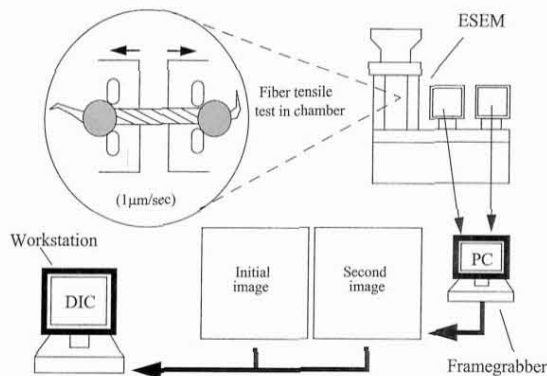
FIG. 1. The experimental set-up for ESEM-based digital image correlation (DIC) evaluation of single fiber microstrains and failure. It consists of a microextensometry located in an ESEM. Single fibers are secured by a free-fiber-alignment ball and socket assembly. Digitally captured images of tensile tests were ported to a workstation for analysis by DIC via a PC-based framegrabber.
