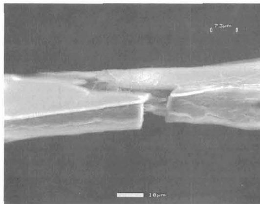
FIG. 3. A single black spruce latewood fiber (low fibril angle) strained to failure. The brush fracture surface is characteristic of fibers with a slow S_2 layer microfibril angle.
