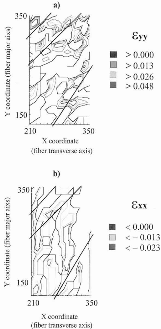
FIG. 7. Quantitative characterization of a) \epsilon_{yy} and b) \epsilon_{xx} in a micro-created region of a wood fiber cell wall. The diagonal lines represent the approximate locations of the cell-wall defect creases. Applied strain = 0.53%. Initial subimage spacing = 13 pixels. Strain tolerance = 0.7%. A distinct Poisson effect was noticeable in all single fiber strain maps.
