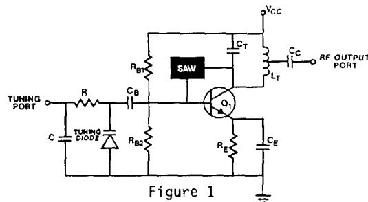
SAW 1-PORT RESONATOR VOLTAGE CONTROLLED OSCILLATOR PIERCE CONFIGURATION
