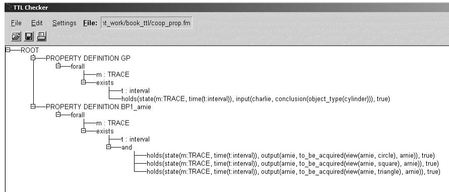
Fig. 5 Screenshot from the TTL Checker Tool
