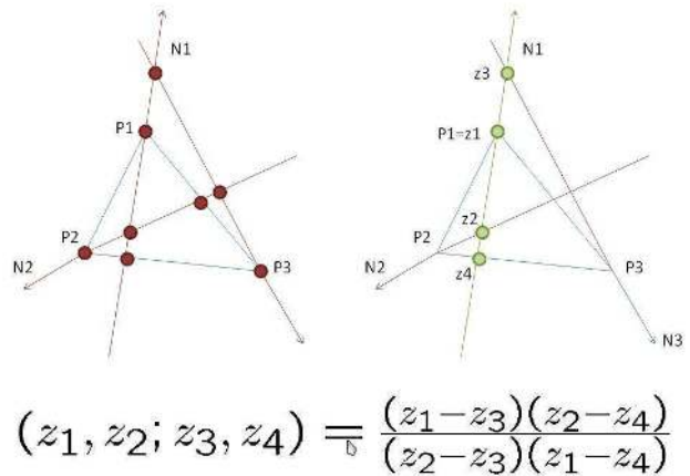
Fig. 5. Left: diagram illustrating the features used in the proposed projective-invariant potential. In order to describe the blue triangle, we build three red lines with four points on each. Right: in order to describe one of these lines (the green one), we denote the four points by z_1 to z_4 (complex numbers). Bottom: we use the cross ratio formula to compute one descriptor for each of the three lines.
