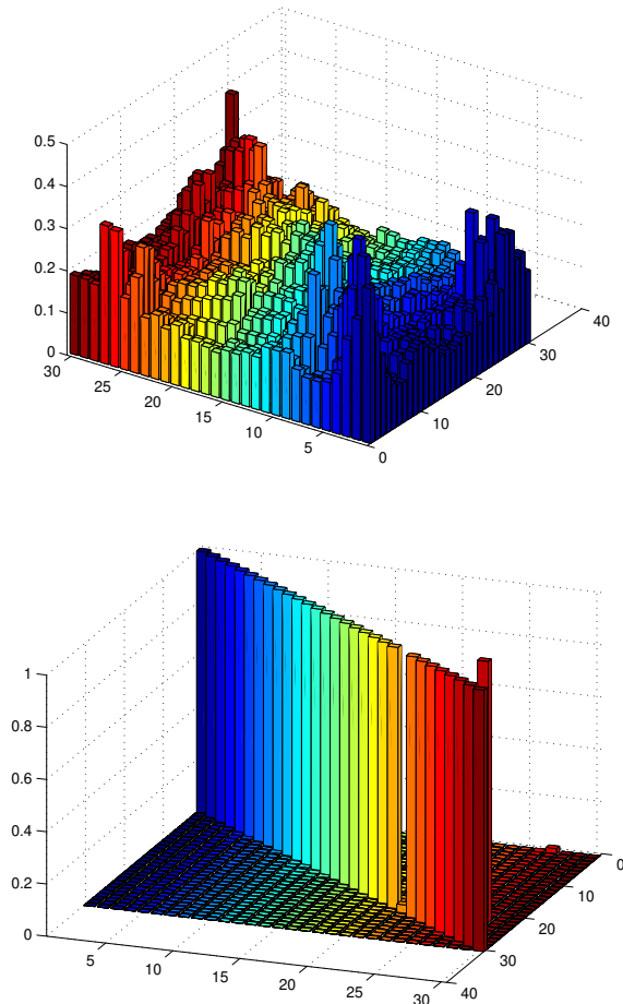
Fig. 3. We run the spectral algorithm to match a random point cloud to a randomly perturbed copy of itself. We show here the resulting assignment matrices by using \ell^2 or \ell^1 -norm constraints (respectively Algorithm 1 and 5). The indexing of the points is made such that for all i , the point i of the first cloud corresponds to the point i of the second cloud. So the perfect assignment matrix should be the identity matrix. The horizontal axes correspond to the coordinates of the assignment matrix and the vertical one to its values. Top: Values of the assignment matrix when the \ell^2 -norm is used. They are hard to project to a matrix in \mathcal{X} , i.e., with values in \{0, 1\} . Bottom: When using the \ell^1 -norm, we obtain directly a very clear assignment matrix with minor adjustments. Indeed, its values are nearly boolean.
