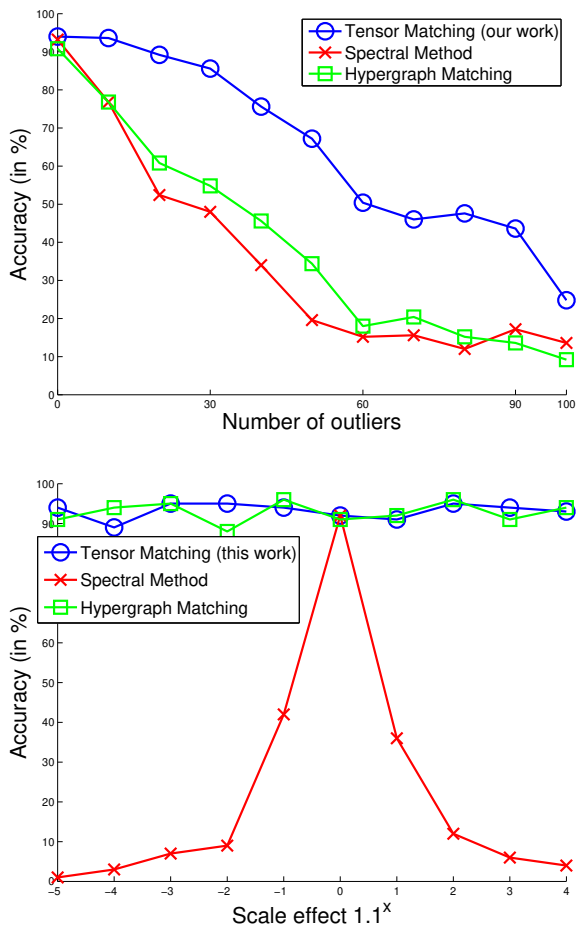
Fig. 7. Top: Accuracy as a function of the number of added outliers. Bottom: Accuracy, as a function of the rescaling. (e.g., x = 2 , correspond to a scaling of 1.1^2 ).
