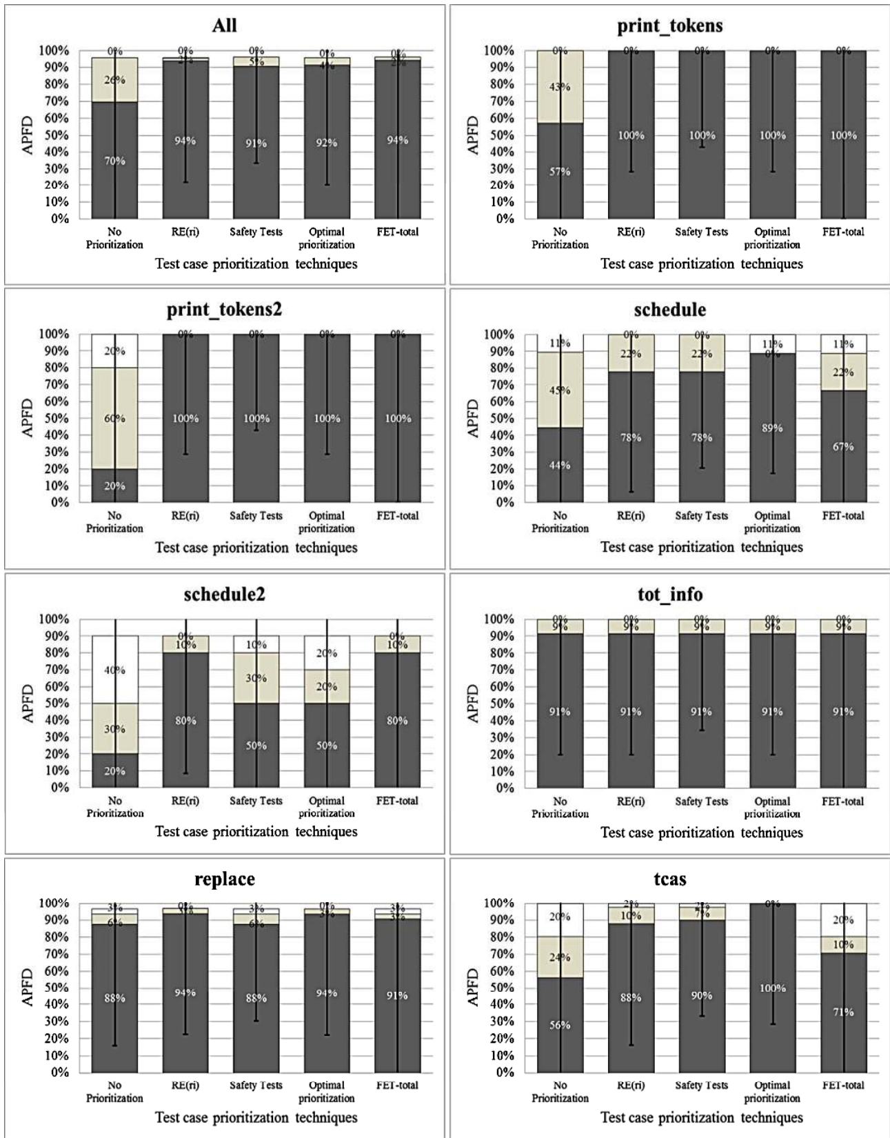
Figure 4. APFD box-plots (vertical axis is APFD score).
