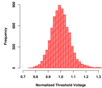
Fig 7: Threshold voltage distribution
