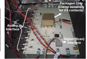
Fig 3: layout of the structure and picture of the test board
