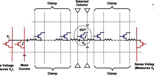
Fig 2: Row sensing for IR drop calibration
