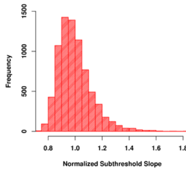
Fig 9: Subthreshold slope distribution
