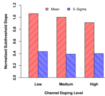
Fig 10: Subthreshold leakage statistics for three different V_T implants
