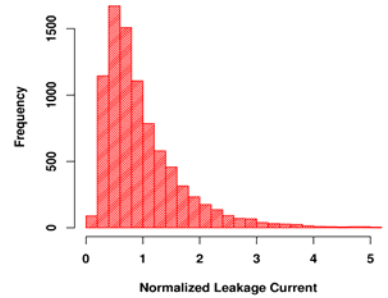
Fig 5: Measured leakage histogram
