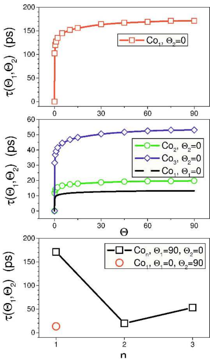
Co on top of Pt(111). Top: n=1 , switching from perpendicular to in-plane, middle: n > 1 , switching from in-plane to perpendicular. Bottom: comparison of the switching times to reach the reorientation transition with respect to the number of Co layers. 215x279mm (600 x 600 DPI)
