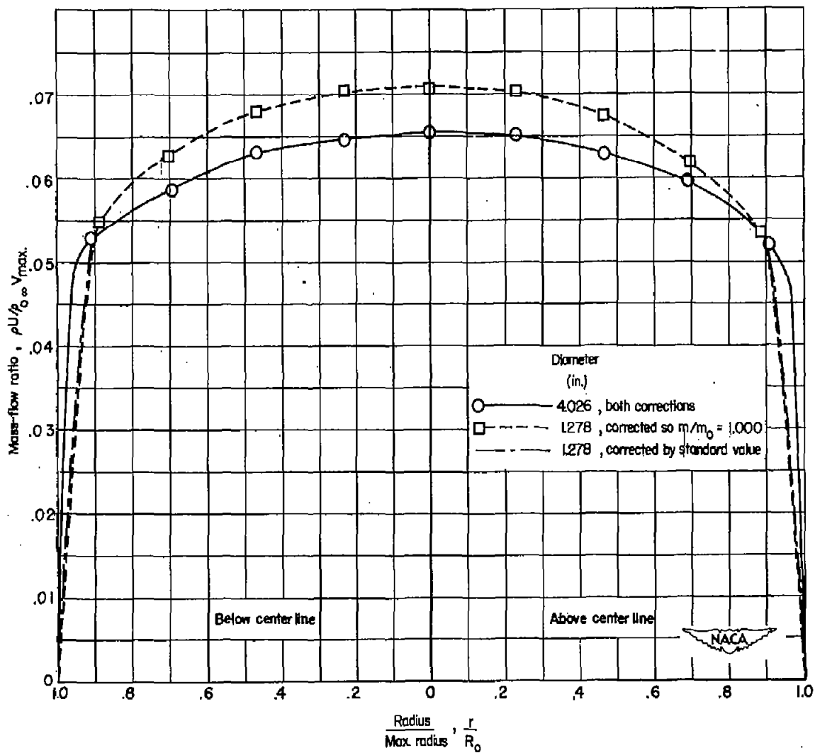
Figure 13.- Mass-flow profiles at rake survey station for configurations 20.82 - 48.1°.
