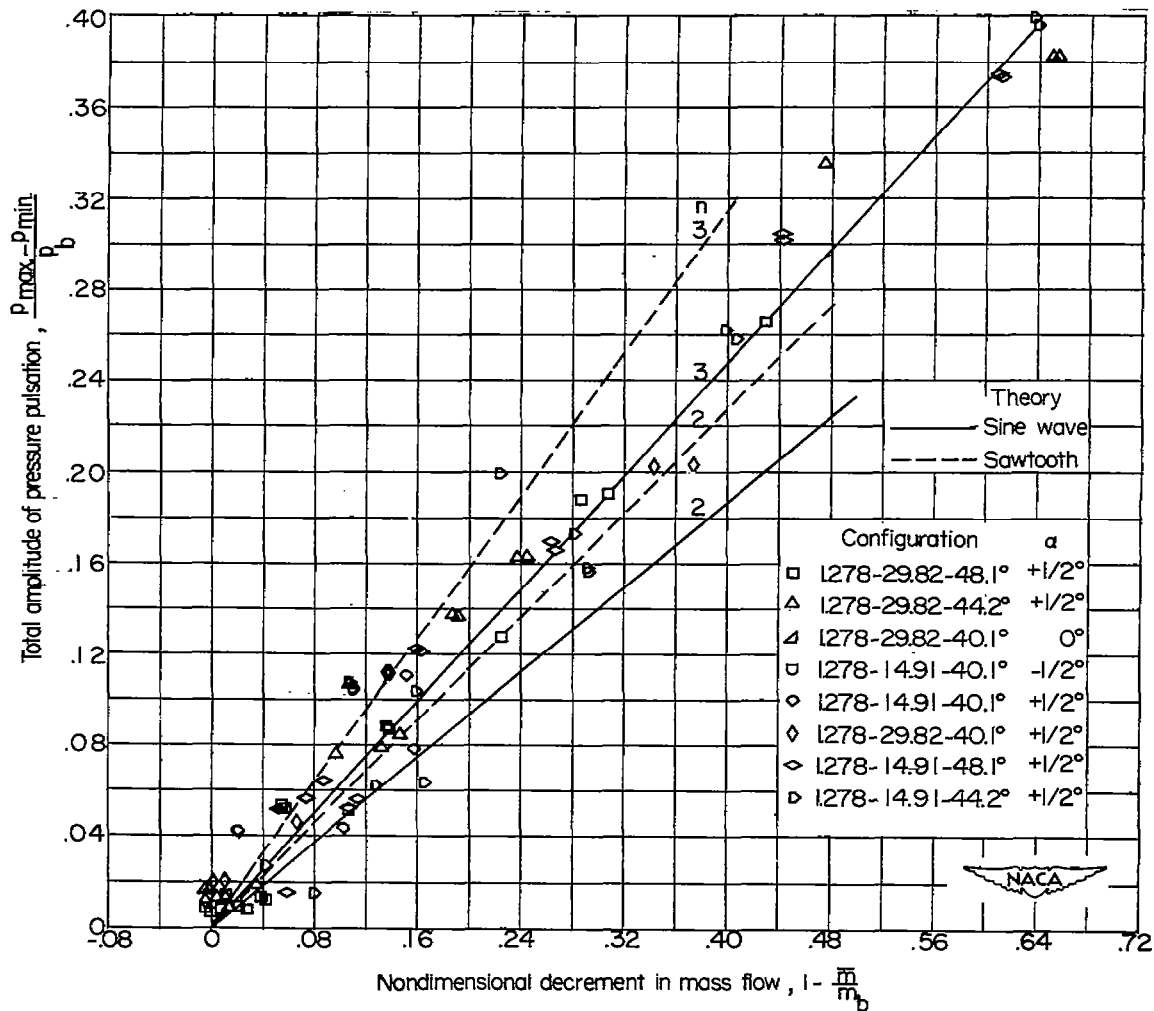
Figure 26.- Total amplitude of pressure pulsations at gage 4 plotted against nondimensional decrement in mass flow from minimum stable flow. Configurations 1.278.
