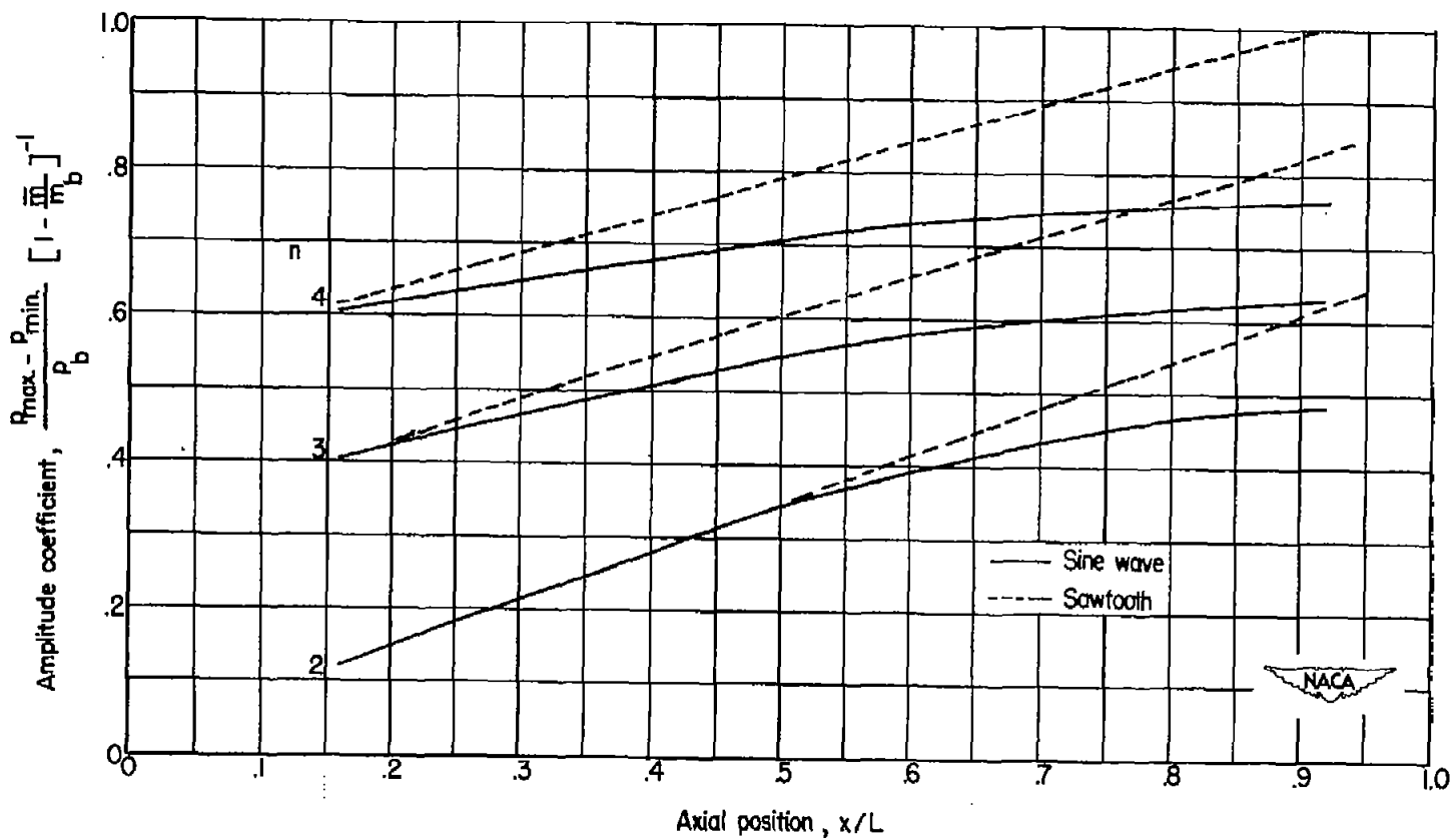
Figure 24.- Variation of pressure amplitude coefficient with axial position for M_D = 0.14 .
