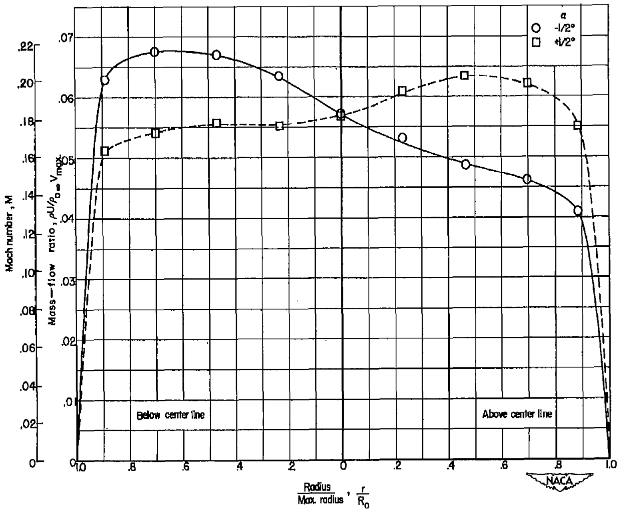
Figure 17.- Mass-flow and Mach number profiles at rake survey station for configuration 1.278 - 14.91 - 40.1° at angles of attack of \pm 1/2^\circ .
