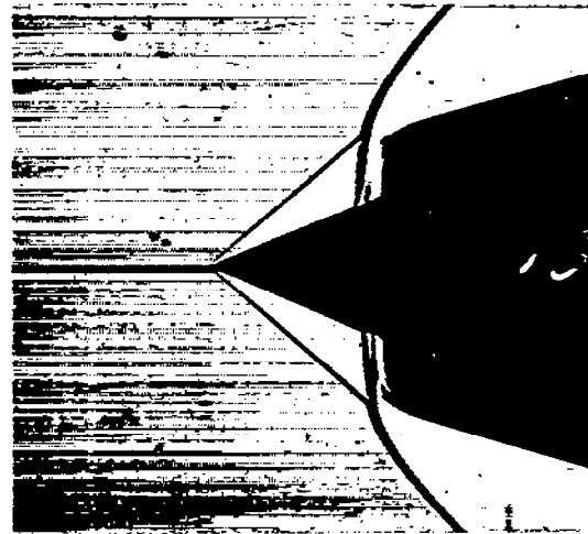
(f) Configuration 1.278-2982-40.1 0 ; \alpha = +1/2^\circ
