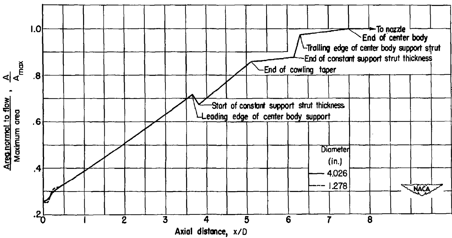
Figure 3.- Local flow area plotted against axial distance from cowling for models tested. Cowling position angle 44.2^\circ .
