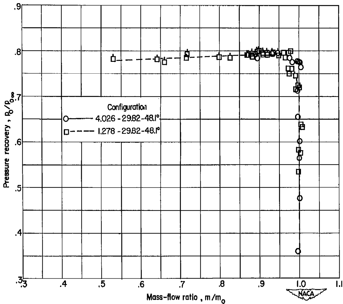
Figure 4.- Curves of pressure recovery plotted against mass-flow ratio for configurations 29.82 - 48.1°. Flagged symbols denote unsteady flow.
