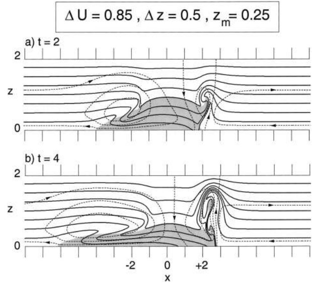
FIG. 6. As in Fig. 4 except \Delta U = 0.85 , \Delta z = 0.5 , and z_m = 0.25 .
