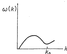
Fig. 1. Schematic feature of phonon eigenfrequencies \omega(k) in a structure disorder system.
