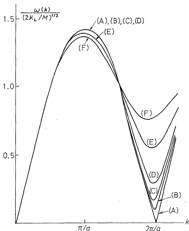
Fig. 4. Phonon eigenfrequencies in a model 1-D structure disorder system (Eq. (6.4)) for various values of \gamma=d/a ; (A): \gamma=0.00 (crystal lattice), (B): \gamma=0.02 , (C): \gamma=0.05 , (D): \gamma=0.10 , (E): \gamma=0.20 and (F): \gamma=0.30 .
