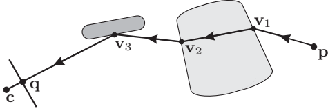
Figure 2. An example light path. The dark gray region denotes a mirror-like object and the light gray region a transparent object. Here, the light path from \mathbf{p} intersects three surfaces before reaching point \mathbf{q} on the image plane, and therefore has three vertices, \mathbf{v}_1 , \mathbf{v}_2 and \mathbf{v}_3 , and four rays. In light-path triangulation, the coordinates of \mathbf{c} , \mathbf{q} and \mathbf{p} are known and the goal is to determine the coordinates and normals of the vertices. By convention, we order vertices and rays along a path according to the direction of light travel.
