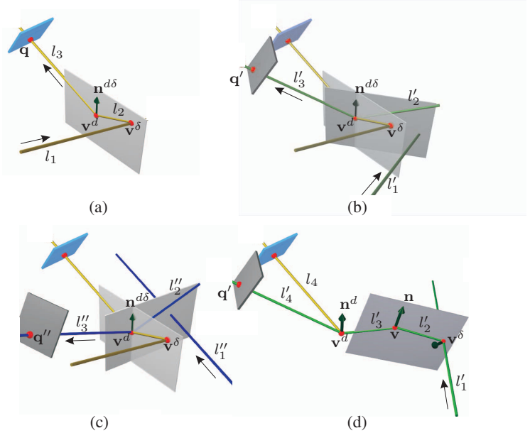
Figure 6. (a)-(c) Path geometries in proof of Proposition 2.
