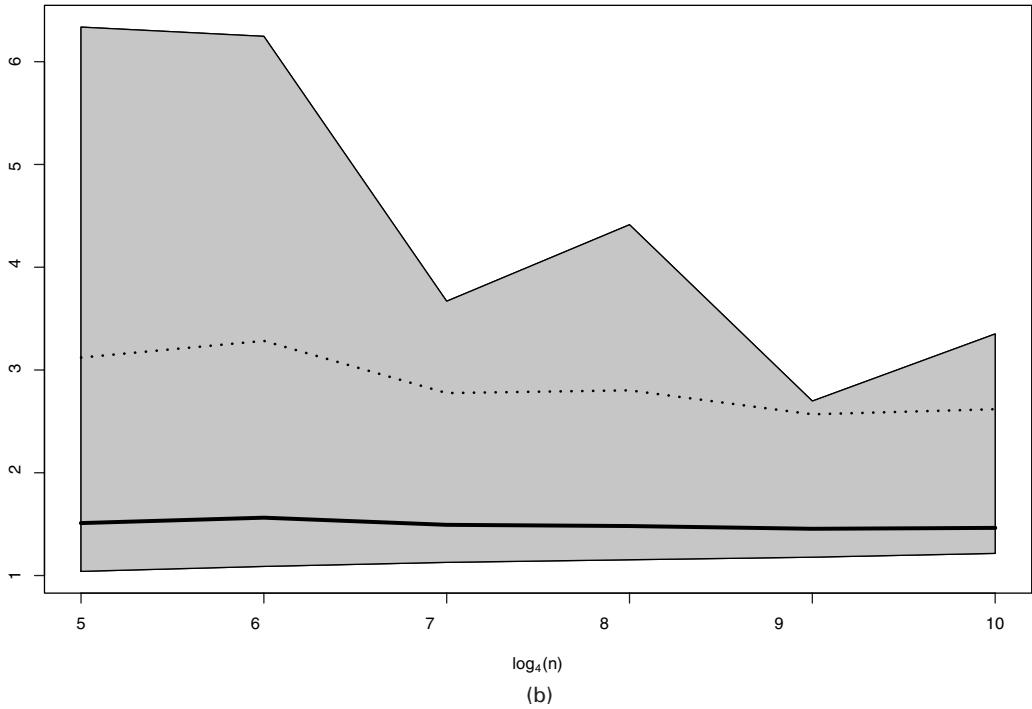
Fig. 2. (a) Contour plot of the density of the logit transform of the \mathcal{N}\{-5, 10, \sigma^2 I_2\} distribution and (b) summary of the successive evaluations of C_\sigma/C_1 = \sigma^2 = 1.5 by averages over the groups \mathcal{G}_n for the logit transform of a single simulated value (x_1, x_2) \sim \mathcal{N}\{-5, 10, \sigma^2 I_2\} : —, average over 100 replications; ■, range of the evaluations; ·····, 2-standard-deviations upper bound
