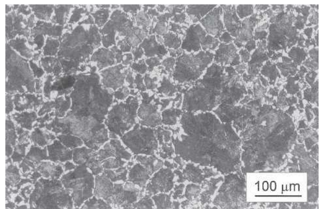
Fig. 17—The as-received microstructure of the hot-rolled AISI/SAE 1045 steel bar consisting of ferrite (white) decorating grain boundary and pearlite (gray) within the grains.
