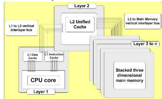
Fig. 2: Schematic view of processor-cache-memory system implemented in 3-D architecture.
