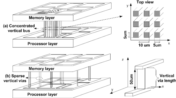
Fig. 3: Schematic view of a vertical bus interconnecting two layers stacked vertically: (a) Concentrated vertical memory bus is easier to route but has large capacitance due to small distance between adjacent vias, (b) Sparse bus has lower capacitance but makes routing complicated.
