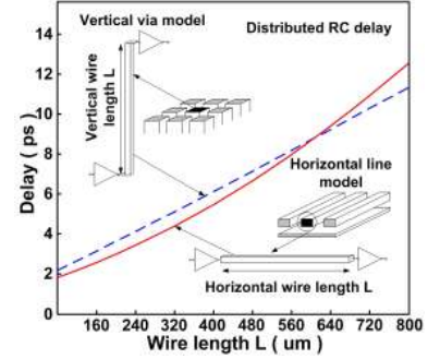
Fig. 4: RC delay comparison for horizontal global interconnect (typical dimension in a 2-D chip [1]) and vertical concentrated bus (see Fig 3(a)) of equivalent lengths. The longest length shown here (800 µm) corresponds to a long stacked via spanning 20 layers. Driver and load device parameters are obtained from [1]. Chip temperature = 105°C.
