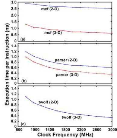
Fig. 7: Execution time per instruction for 2-D versus 3-D chip for (a) mcf benchmark (highly memory intensive), (b) parser benchmark (less memory intensive) and (c) twolf benchmark (least memory intensive), as a function of clock frequency.
