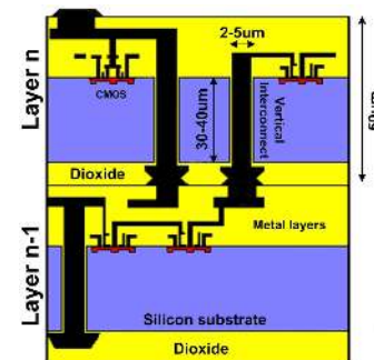
Fig. 1: Cross-sectional view of an n-layer vertically stacked active layers interconnected through vias.
