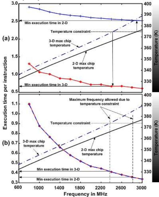
Fig. 9: Execution time per instruction and maximum chip temperature as a function of operating frequency for 2-D and 3-D chip for (a) highly memory intensive ( mcf ) application and (b) less memory intensive ( twolf ).
