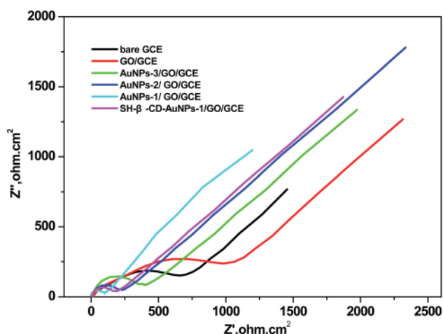
Fig. 3 Electrochemical impedance spectroscopy results of the different modified electrodes in 5 \times 10^{-6} \text{ mol L}^{-1} \text{ Fe}(\text{CN})_6^{3-/4-} containing 0.1 M KCl solution (pH = 7.0).
