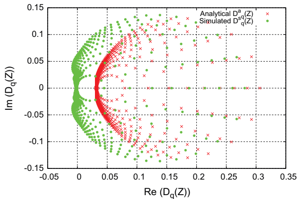
(a) M/G/1
