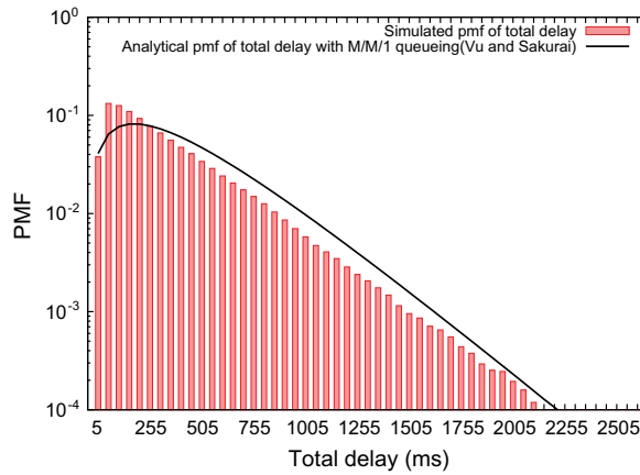
(c) Total delay PMF for 2-hop
