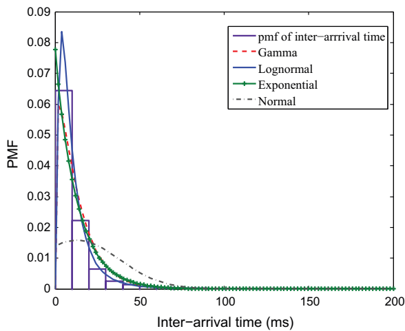
(a) n = 5
