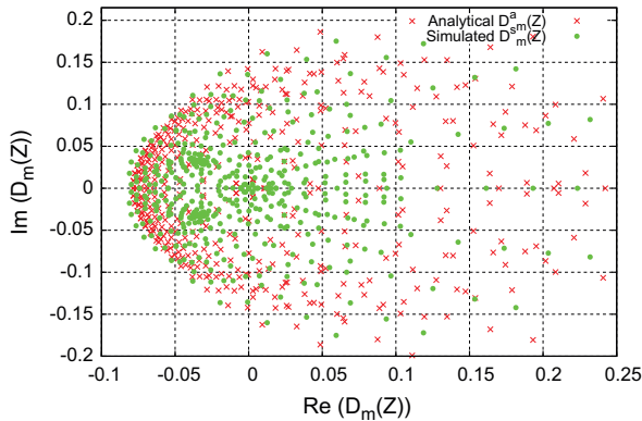
(a) MAC Modeling error: D_m^a(Z) vs. D_m^s(Z) for n = 5
