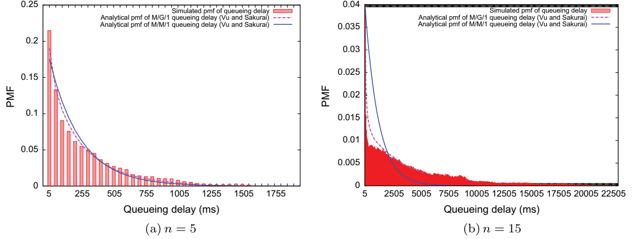
Fig. 5. Analytical queueing delay PMFs for M/M/1 and M/G/1 queues vs. simulations.
