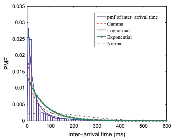
(b) n = 30
