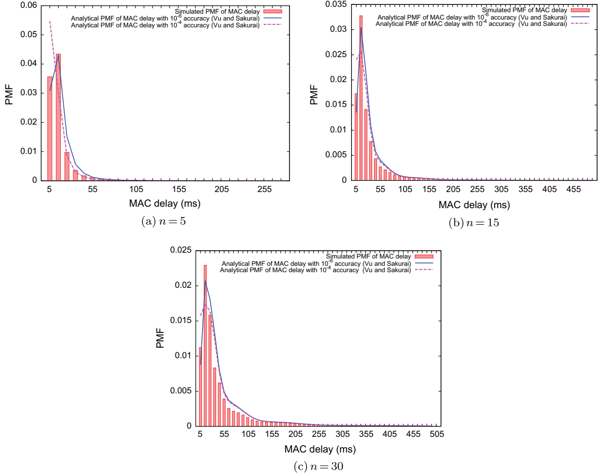
Fig. 4. MAC delay PMF for different accuracies using Vu and Sakurai's LP formula.
