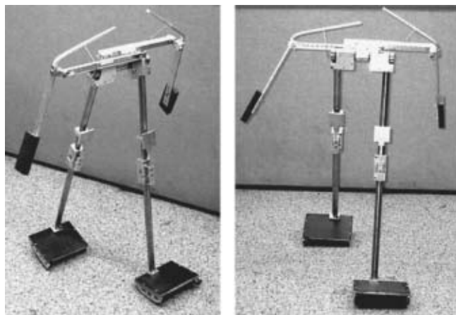
Fig. 3. Our two-legged, kneed, passive-dynamic walking robot. The counter-swinging arms are attached rigidly to their opposing legs. Note that the right arm swings forward and out as the left leg swings forward.
