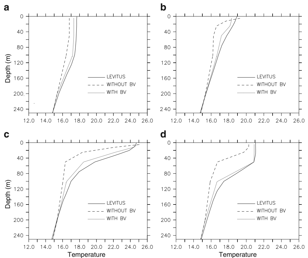
Fig. 8 Comparisons among the simulated temperature from the uncoupled ( dashed ) and coupled ( dotted ) POM and the Levitus data ( solid ) at (35° N, 30° W) in a February, b May, c August, and d November
