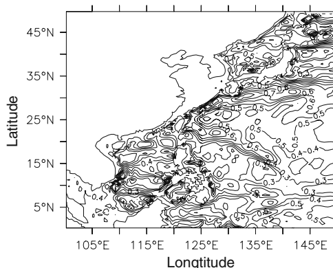
Fig. 12 The stream function (in sverdrup) of wave-driven-only circulation in the Northwest Pacific in July
