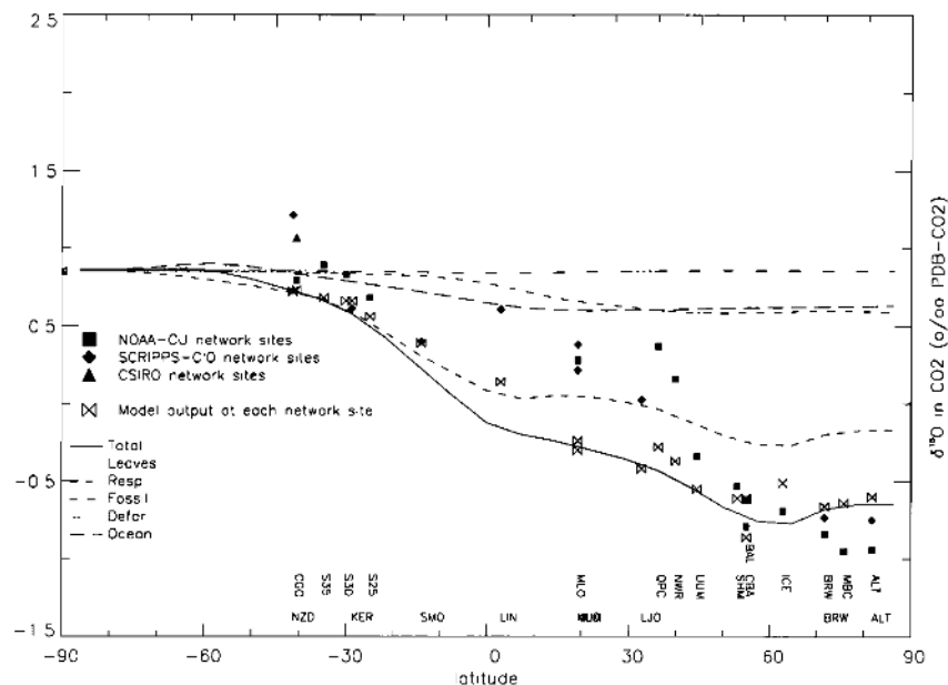
Figure 3. Zonally averaged latitudinal profile of \delta^{18}\text{O} in \text{CO}_2 at the surface. The different curves separate the exchange with leaves, soils, ocean, fossil emissions, and biomass burning. Note that the \delta^{18}\text{O} profiles pertaining to each reservoir are not additive but rather combine linearly to yield the resultant \delta^{18}\text{O} curve in solid line. Solid symbols correspond to the \delta^{18}\text{O} simulated at the precise location of the air sampling sites and are the average of atmospheric data measured on flask samples by NOAA-CU (squares), Scripps-CIO (diamonds), and by CSIRO (triangles). At least 2 years of data have been averaged in the atmospheric measurements shown here.
