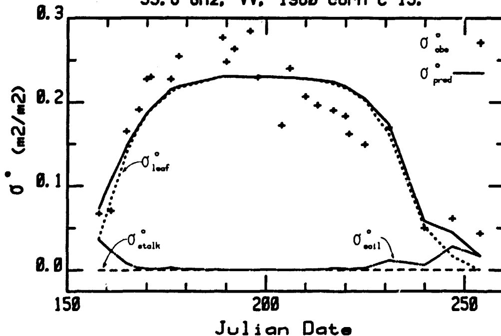
Figure 4.4d. Comparison of predicted and observed \sigma^{\circ} vs date for 35.6 GHz, VV, 1980 corn C-13.
