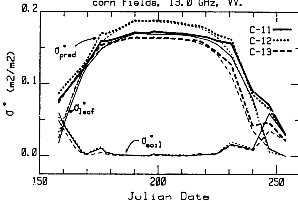
Figure 4.5b. Comparison of predicted \sigma^{\circ} vs date for all 1980 corn fields, 13.0 GHz, VV.
