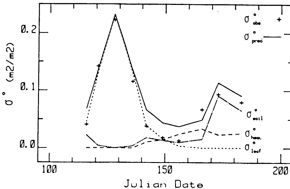
Figure 4.1b. Comparison of predicted and observed \sigma^{\circ} vs date for 13.0 GHz, VV, 1979 wheat W-41.
