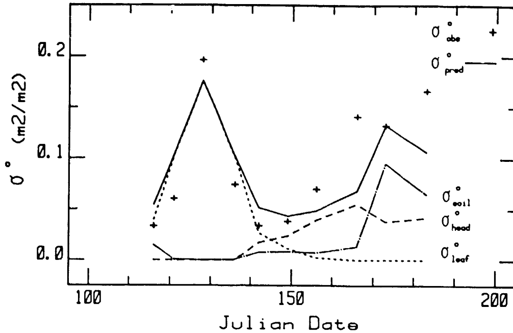
Figure 4.1a. Comparison of predicted and observed \sigma^{\circ} vs date for 8.6 GHz, VV, 1979 wheat W-41.
