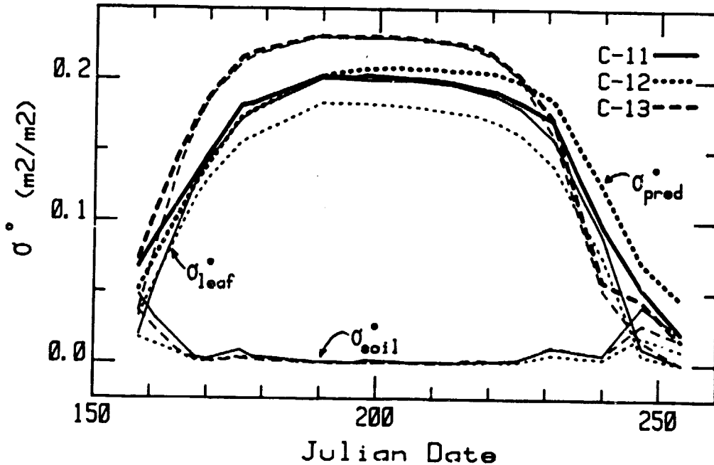
Figure 4.5d. Comparison of predicted \sigma^0 vs date for all 1980 corn fields, 35.6 GHz, VV.
