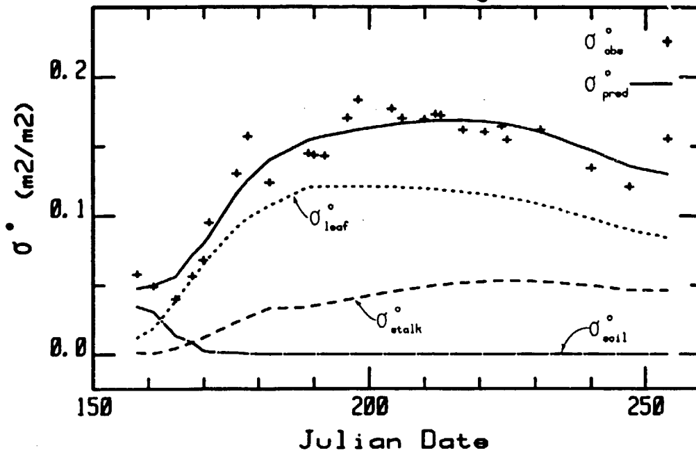
Figure 4.2c. Comparison of predicted and observed \sigma^{\circ} vs date for 17.0 GHz, VV, 1980 sorghum S-33.
