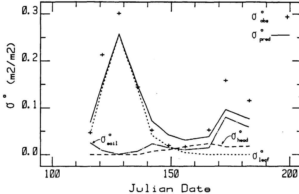
Figure 4.1c. Comparison of predicted and observed \Sigma^{\circ} vs date for 17.0 GHz, VV, 1979 wheat W-41.
