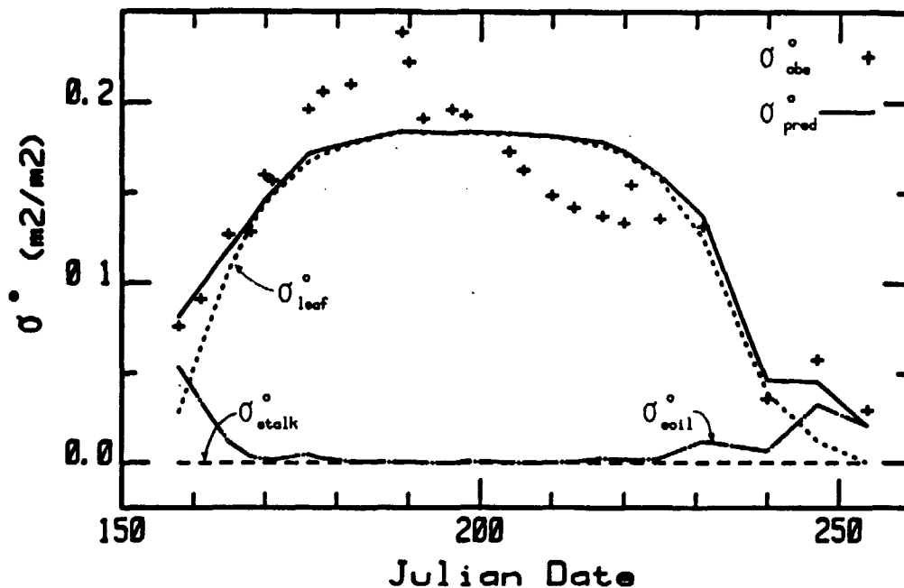
Figure 4.4c. Comparison of predicted and observed \sigma^{\circ} vs date for 17.0 GHz, VV, 1980 corn C-13.
