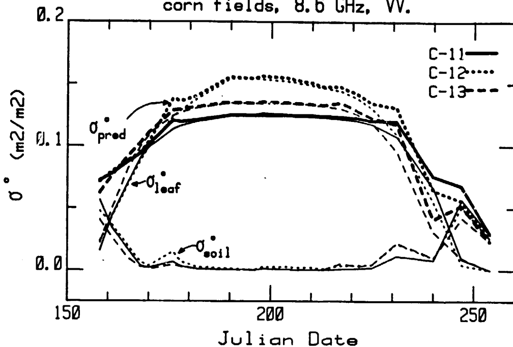
Figure 4.5a. Comparison of predicted \sigma^{\circ} vs date for all 1980 corn fields, 8.6 GHz, VV.
