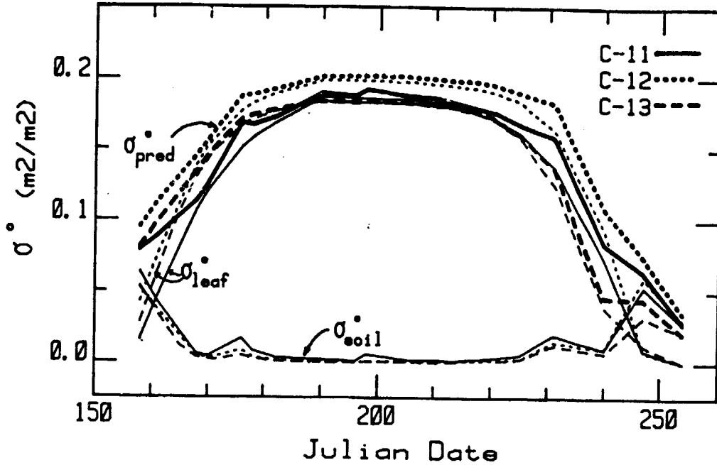
Figure 4.5c. Comparison of predicted \sigma^0 vs date for all 1980 corn fields, 17.0 GHz, VV.
