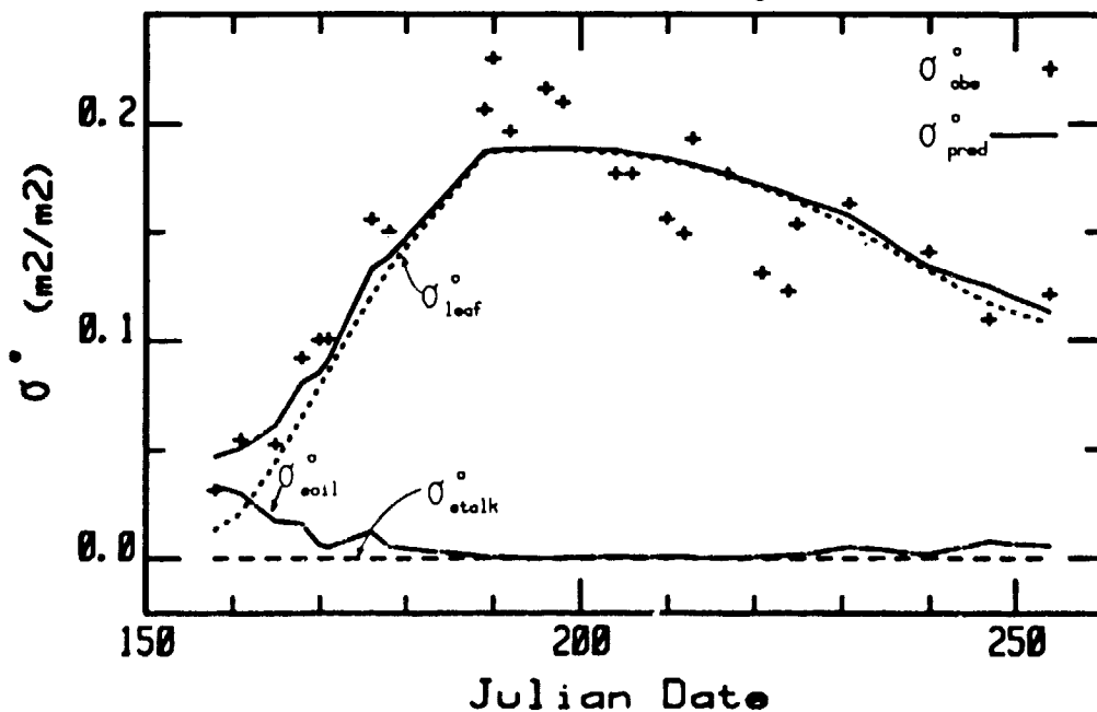
Figure 4.2d. Comparison of predicted and observed \sigma^{\circ} vs date for 35.6 GHz, VV, 1980 sorghum S-33.
