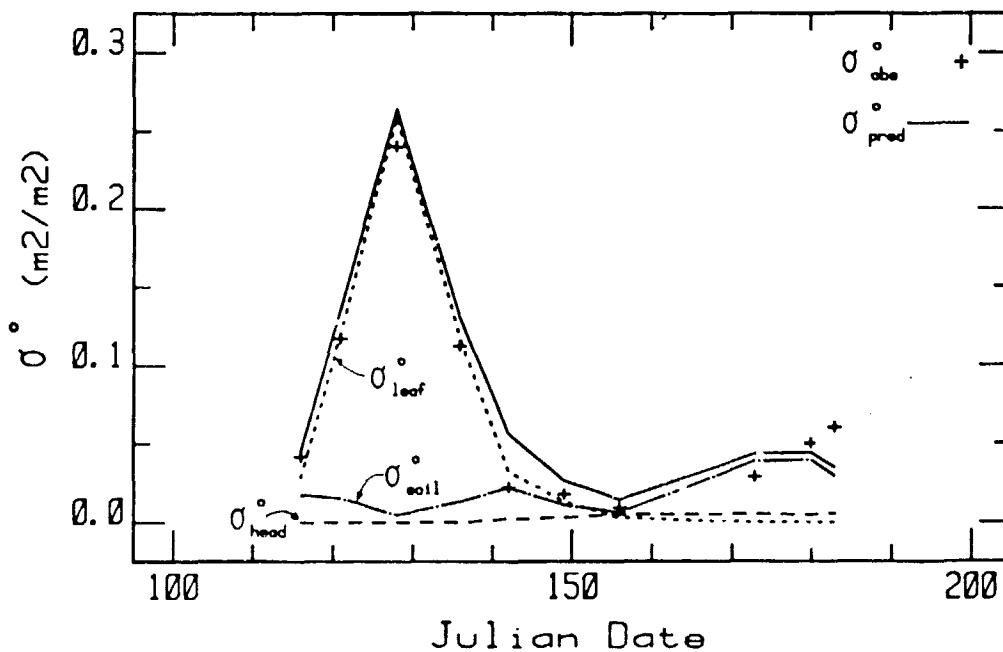
Figure 4.1d. Comparison of predicted and observed \Sigma^{\circ} vs date for 35.6 GHz, VV, 1979 wheat W-41.
