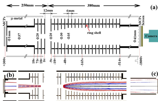
FIG. 2. (Color online) (a) Geometric diagram of the velocity focusing optics and dual TOF tubes in present TPEPICO imaging spectrometer; (b) simulated trajectories of the threshold (in black) and 50 meV (in red) energetic electrons; (c) simulated trajectories of ions with zero (in black), 0.3 eV (in blue), and 0.8 eV (in red) kinetic energy. In all simulations above, the extraction field is 15 \text{ V cm}^{-1} .
