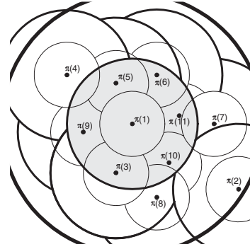
Figure 2: A possible hierarchical cut decomposition output by the algorithm. The varying thicknesses indicate cuts at different levels.
