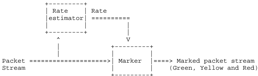
Figure 1. Block diagram for the TSWTCM
