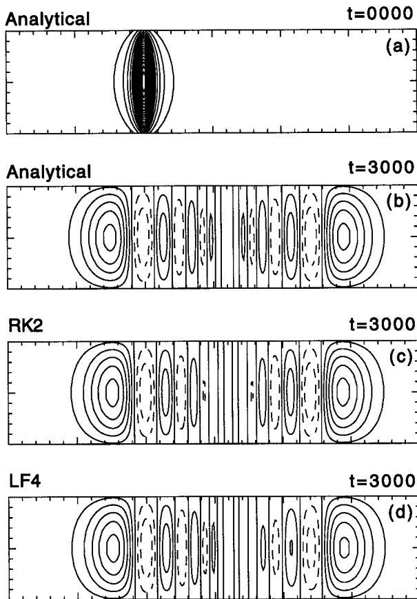
FIG. 3. (a) Perturbation \theta at t = 0 for the nonhydrostatic gravity wave test, plotted with a contour interval of 10^{-3} K. The plotted domain is 300 km by 10 km. (b) Analytical solution for perturbation \theta at t = 3000 s, plotted with a contour interval of 0.5 \times 10^{-3} K, for the analytic solution. (c) Perturbation \theta at t = 3000 s for the RK2 model. (d) Same as (c), except for the leapfrog model.
