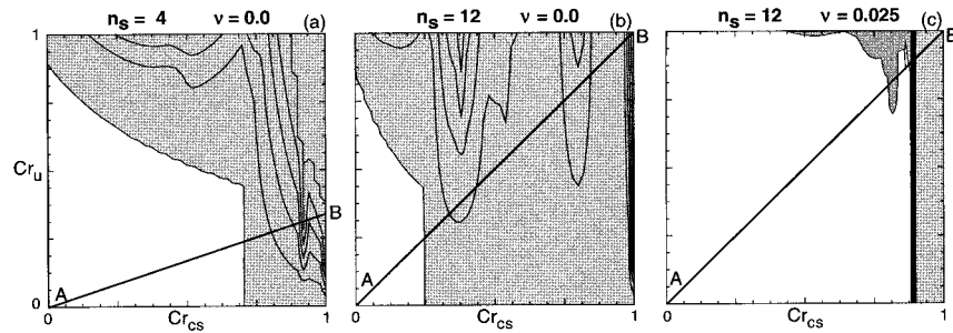
FIG. 2. Maximum amplification factor for the split-explicit third-order RK2 scheme. The contour interval is 0.1 and Cr_u and Cr_{cs} are the advective and sound speed Courant numbers, respectively; (a) n_s = 4 , (b) n_s = 12 , (c) n_s = 12 , with a divergence damping coefficient \alpha = 0.025 . The lines AB are plotted using U/c_s = 1/12 , and shaded regions indicate where the amplification factor is greater than 1.
