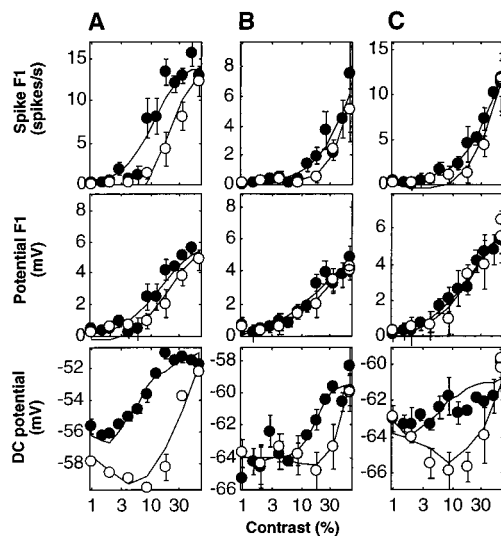
Fig. 3. Effects of contrast adaptation as measured with the ramp method (13). For three simple cells (A to C), the F1 component of the spike response (top), the F1 component of the membrane potential (middle), and the DC component of the membrane potential (bottom) are shown. The data in (A) are taken from the same cell as Fig. 1. Stimuli lasting 4 s were presented, the first at 1% contrast and each successive one at greater contrasts up to 64% (●). Contrast was then successively lowered back to 1% (○). The curves are fits of a model in which adaptation depends on the past responses of the cell. The adapted responses R_A are given by a hypothetical unadapted response R (described by Eq. 1) minus the sum of the five previous responses, each weighted by a factor that decayed exponentially in time:
