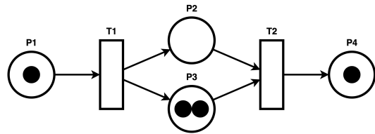
Figure 2: Petri nets Model Example
