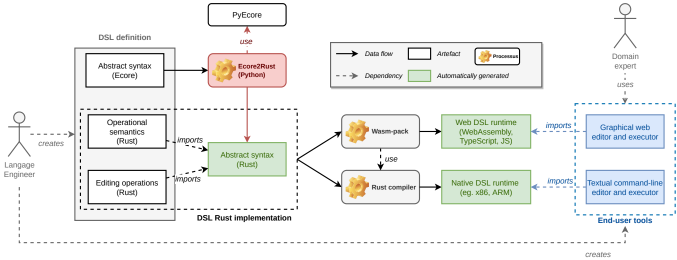
Figure 3: Approach Overview
