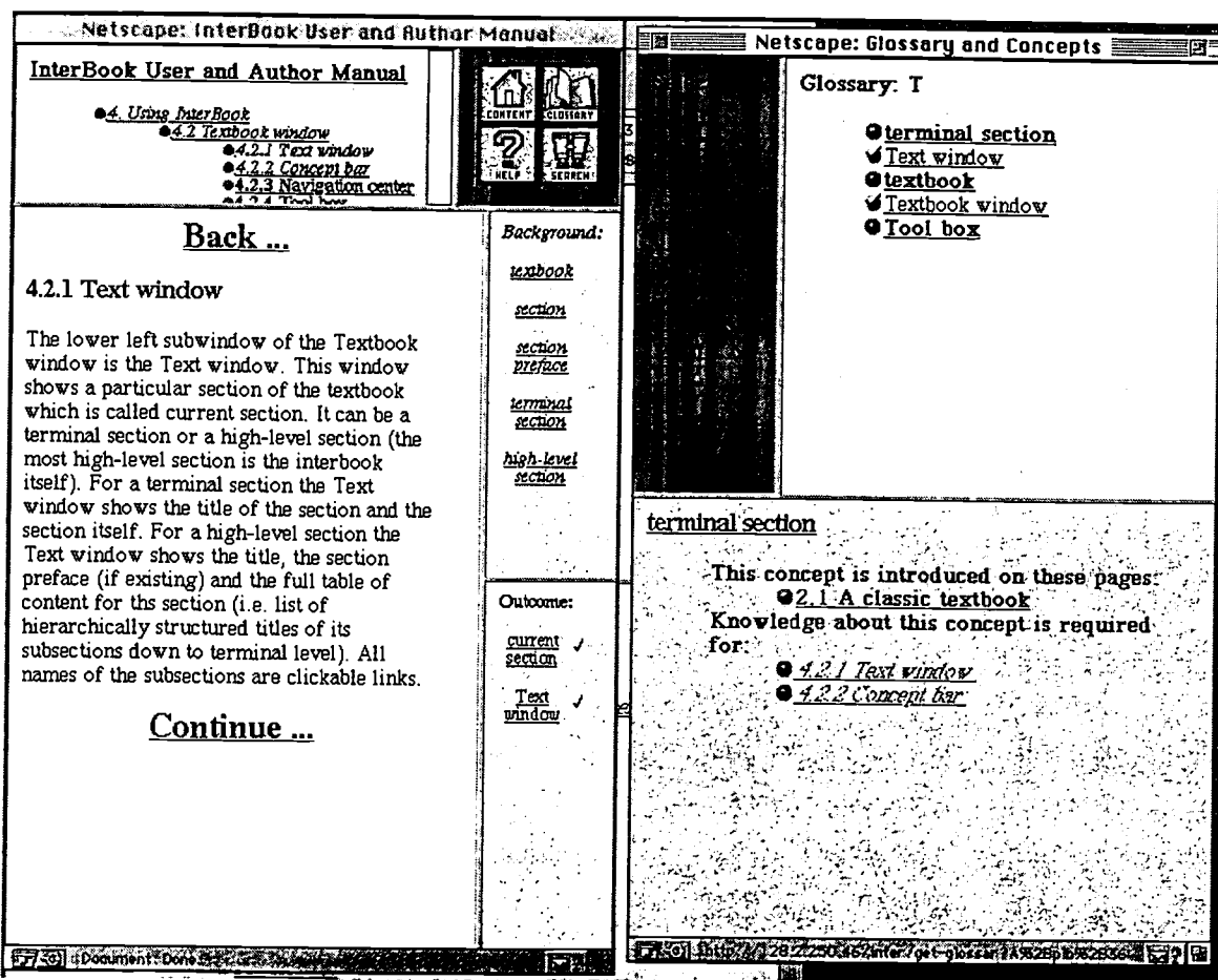
Figure 1: Textbook and Glossary windows of InetrBook
