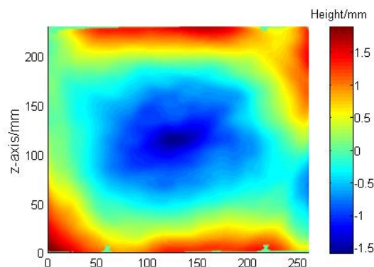
Fig. 5 The chart of surface residual error
