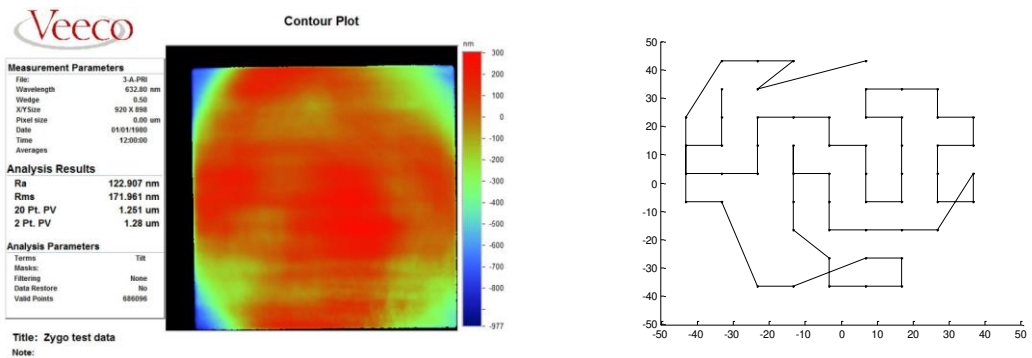
(a) Surface shape of workpiece (PV=1.28um)
