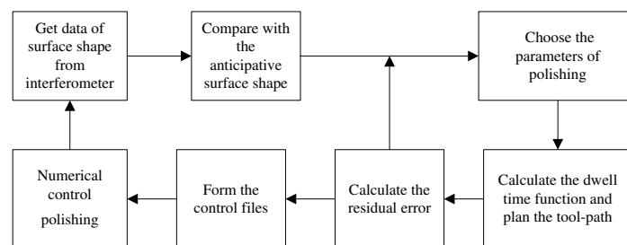
Fig. 1 Process flow chart of CCOS
