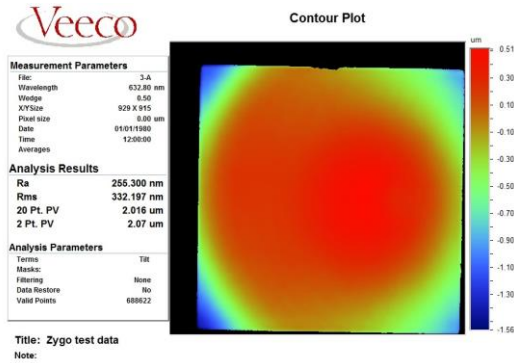
Fig. 10 Initial surface shape of workpiece (PV=2.07um)
