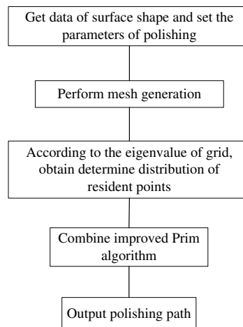
Fig. 4 The flow chart of generating polishing path
