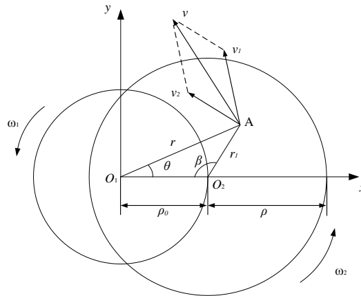
Fig. 8 Motion of polishing tool in CCOS
