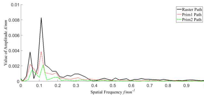
Fig. 15 The spectrum diagram of workpiece after three processing experiments
