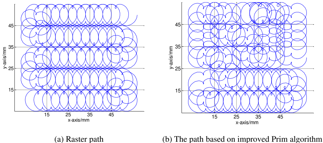
Fig. 10 The trajectories of the point A in high-speed condition
