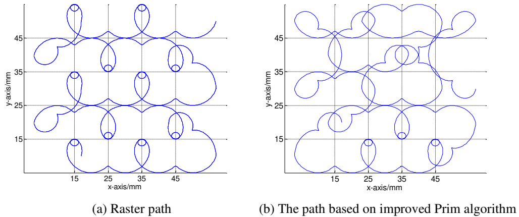
Fig. 9 The trajectories of the point A in low-speed condition
