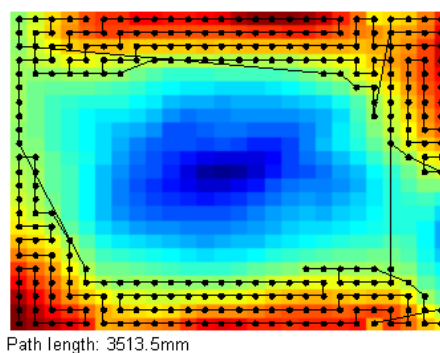
Fig. 7 The path based on improved Prim algorithm
