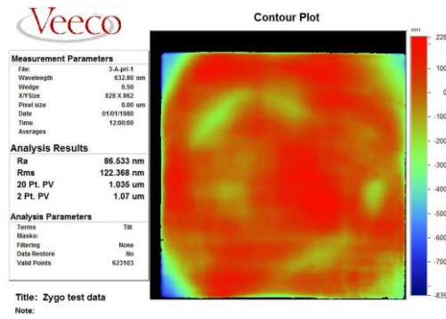
Fig. 14 The third processing experiment with path based on improved Prim algorithm: surface shape of workpiece (PV=1.28um)
