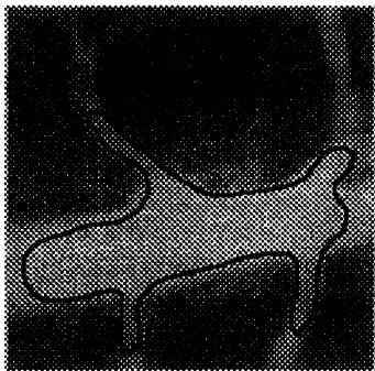
(g) Initialization 3
