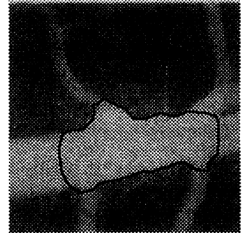
(i) 1000 iterations
