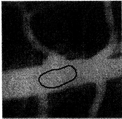
(a) Initialization
