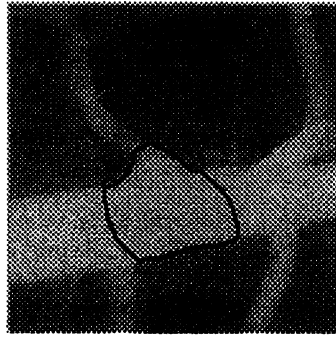
(b) 500 iterations
