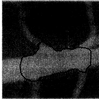
(h) 500 iterations
