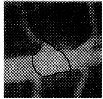
(c) 1000 iterations
