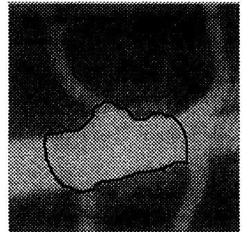
(f) 1000 iterations
