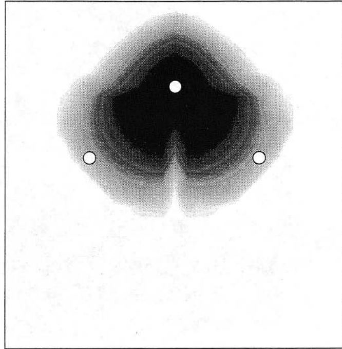
Figure 11: Sample problem 1: Grout content immediately after second injection
