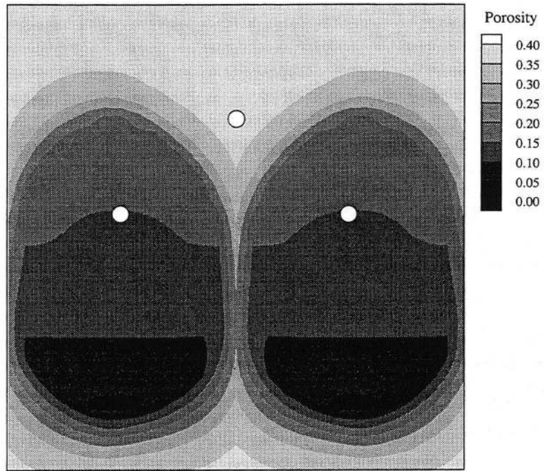
Figure 9: Sample problem 1: Porosity distribution after first solidification
