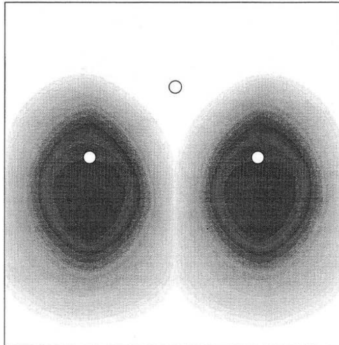
Figure 8: Sample problem 1: Grout content at t = 5 hrs
