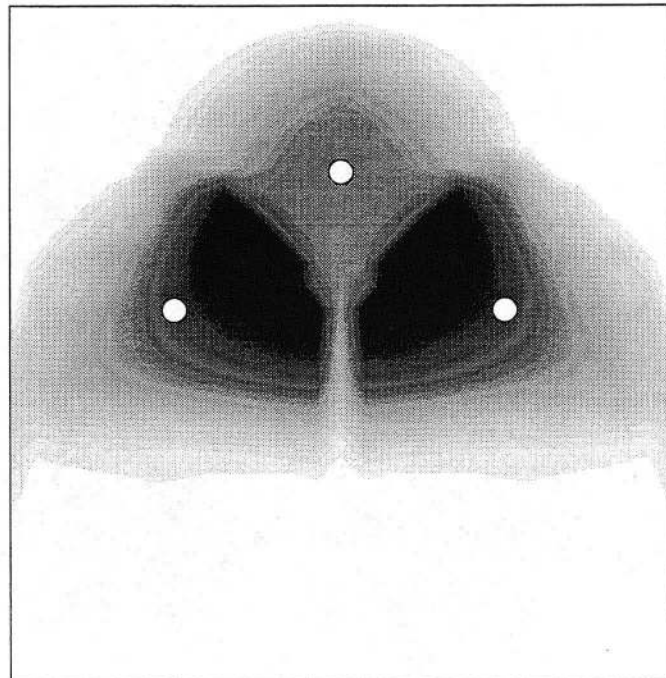
Figure 12: Sample problem 1: Grout content at t = 10 hours
