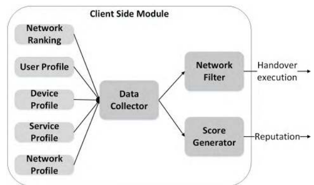
FIGURE 4. Client module.
