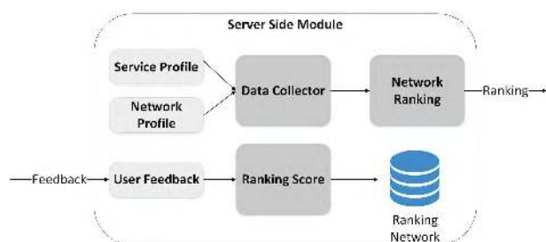
FIGURE 7. Server module.
