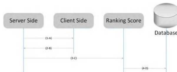
FIGURE 8. Server procedures.
