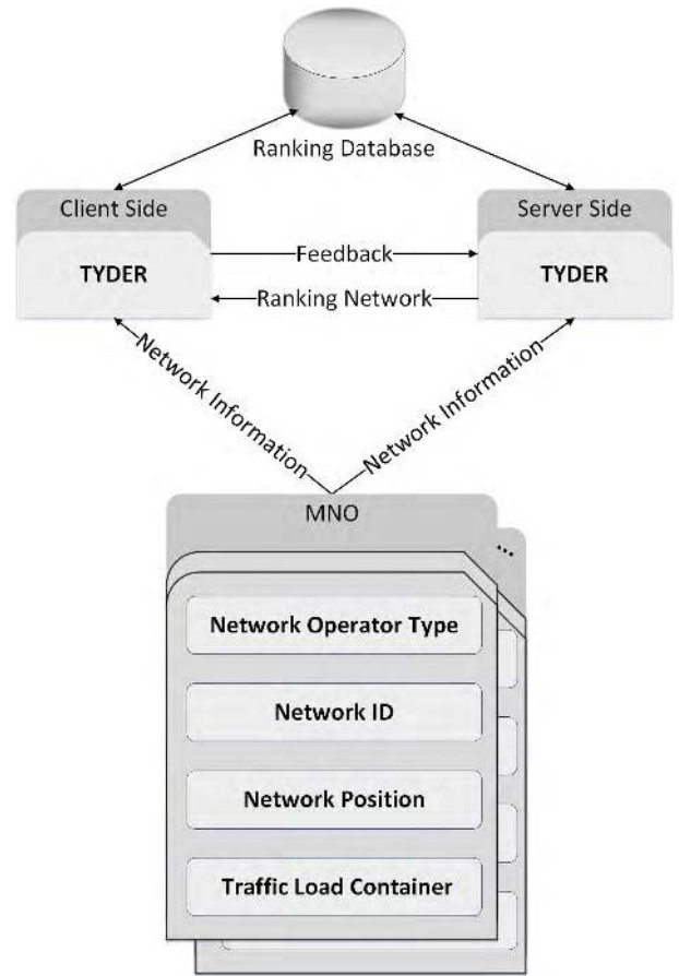
FIGURE 2. TYDER architecture.
