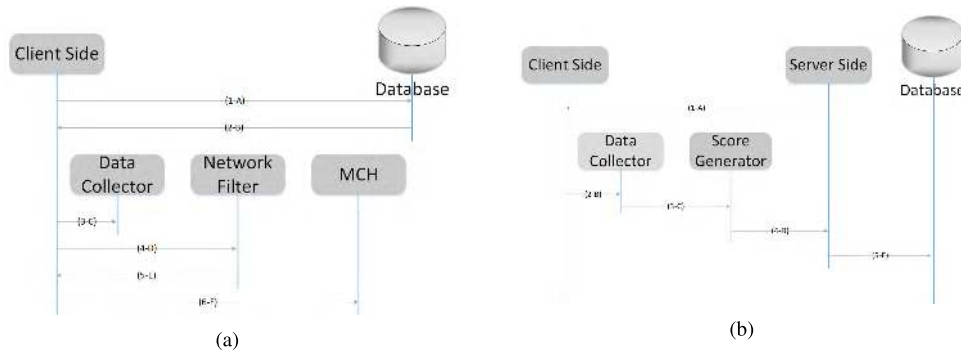
FIGURE 5. Client procedures.
