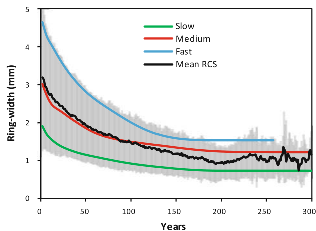
Fig. 13 Three age-aligned, signal free, RCS curves for slow, medium, and fast growth rate trees, with mean RCS and its \pm 1 standard deviation (shading)
