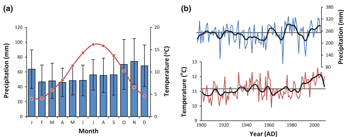
Fig. 2 Regional climate data plots of a monthly mean Central England Temperature (CET) and gridded (49–53°N, 0–2°E) precipitation with \pm 1 standard deviation; b associated MAMJJ time series
