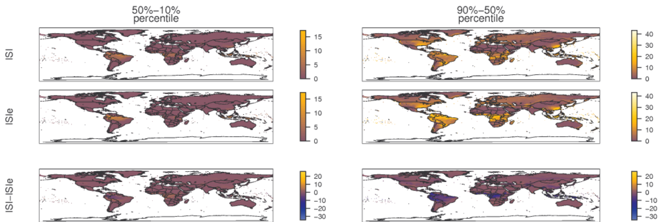
Fig. 10. The lower (50–10 %) and upper (90–50 %) inter-percentile range of the April daily precipitation from 1960 to 1999 are shown for the ISI-MIP dataset (ISI) and with the extended version of the algorithm (ISIE). In addition the differences of both version are shown. The inter-percentile ranges are analogues to Fig. 8. Colours refer to precipitation in \text{mm day}^{-1} . Difference values outside the range of the shown colourbars are white in order to increase visibility of the map (over land this affects only few small areas).
