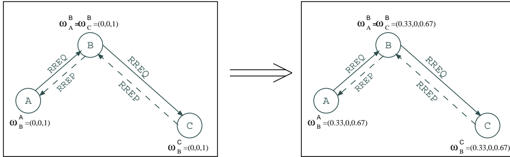
Figure 4. Initialization for TAODV
