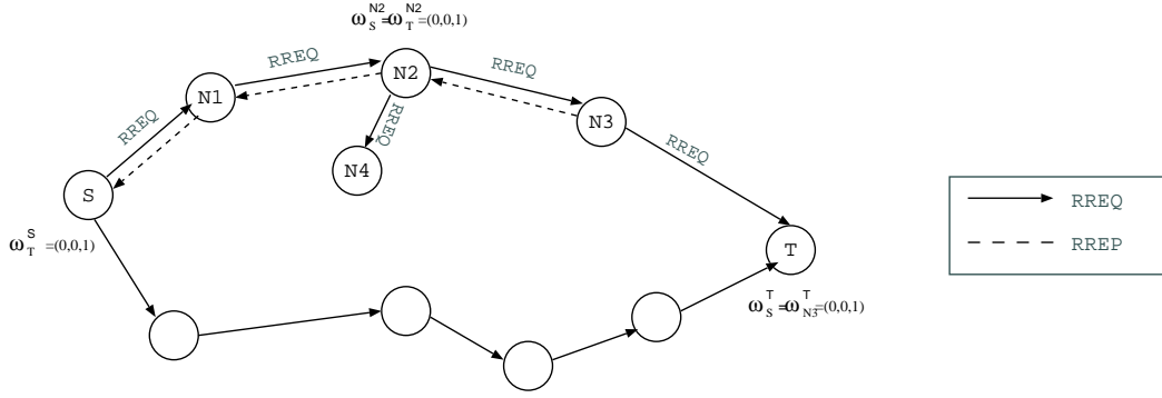
Figure 5. An Example for Trusted Routing Discovery
