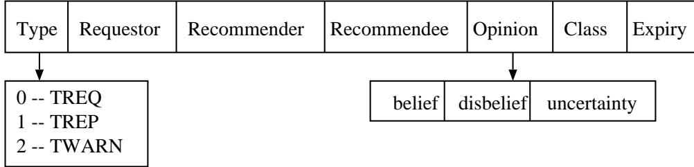
Figure 3. Message Structure of Trust Recommendation Protocol
