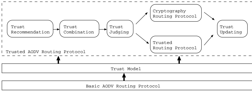
Figure 1. Framework of the Trusted AODV (TAODV)
