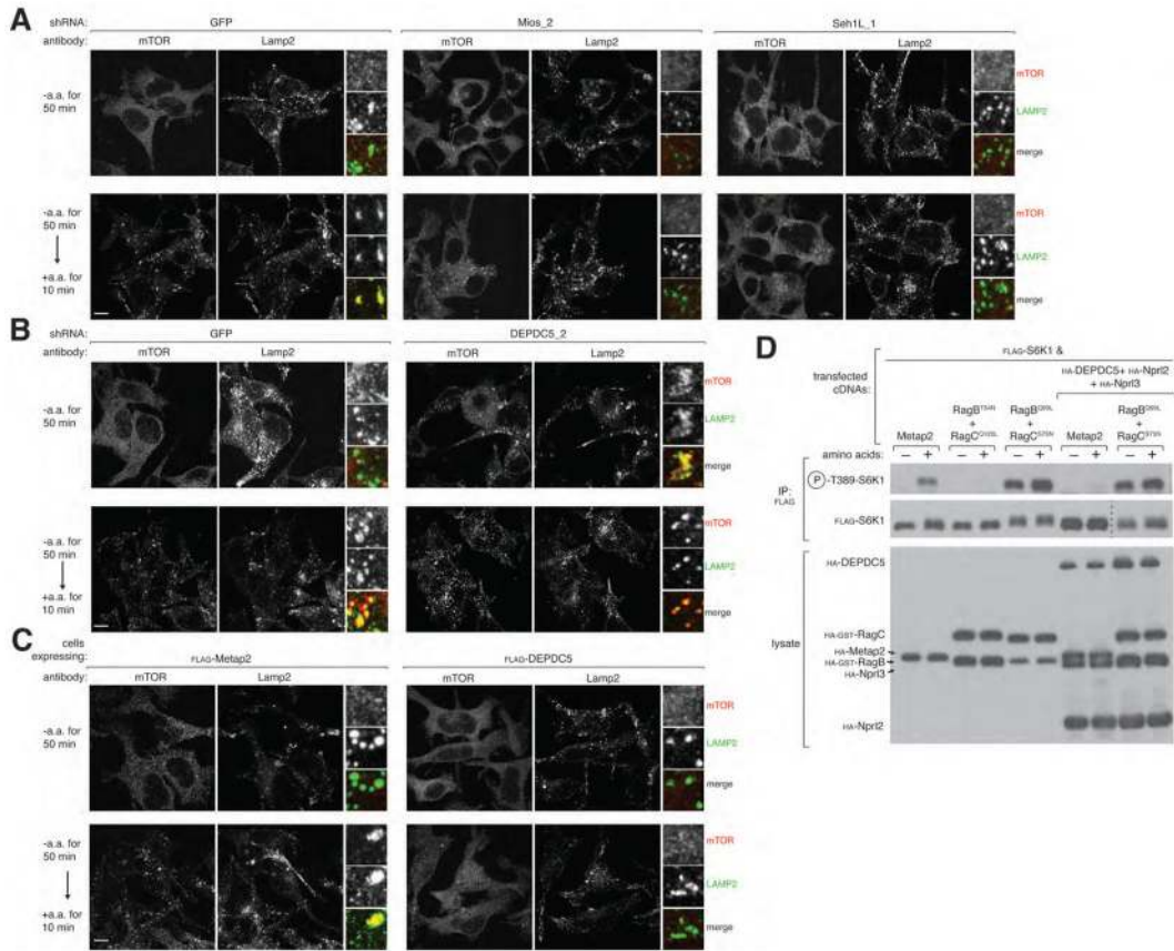
Figure 3. GATOR regulates mTORC1 localization to the lysosomal surface and functions upstream of the Rag GTPases. (A) RNAi-mediated depletion of the GATOR2 components Mios and Seh1L prevents amino acid-induced mTOR lysosomal translocation. HEK-293T cells expressing the indicated shRNAs were starved or starved and restimulated with amino acids for the specified times prior to co-immunostaining for mTOR (red) and Lamp2 (green). (B) Reduced expression of DEPDC5 in HEK-293T cells results in constitutive mTOR localization to the lysosomal surface. HEK-293T cells treated with the indicated lentiviral shRNAs were processed as described in (A) . (C) Images of HEK-293T cells stably expressing FLAG-DEPDC5 starved for or starved and restimulated with amino acids. Cells were processed as described in (A) . In all images, insets show selected fields that were magnified five times and their overlays. Scale bar equals 10 \mu M. (D) GATOR1 functions upstream of the nucleotide binding state of the Rags. HEK-293T cells transfected with the indicated cDNAs in expression vectors were starved of amino acids for 50 min or starved and restimulated with amino acids for 10 min. The indicated proteins were detected by immunoblotting.
