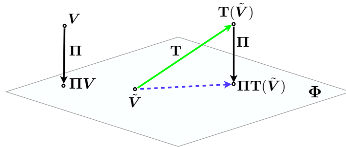
Figure 2.3: A geometric interpretation of what Bellman Residual Minimization (solid green) and Projected Bellman Residual Minimization (dashed blue) minimize [akin to Lagoudakis and Parr, 2003]. \Pi is the projection operator based on the steady state distribution \mathbf{d} , mapping every point to its orthogonal projection on the span of \Phi shown as a 2D plane. \mathbf{T} is the Bellman operator. The ideal approximation is shown by \Pi V , yet it is impractical since V is not known.
