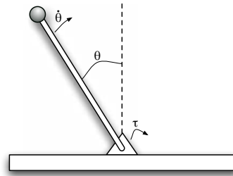
Figure 4.3: The Inverted Pendulum domain: The task is to maintain the balance of a pendulum using torque values applied to the base.
