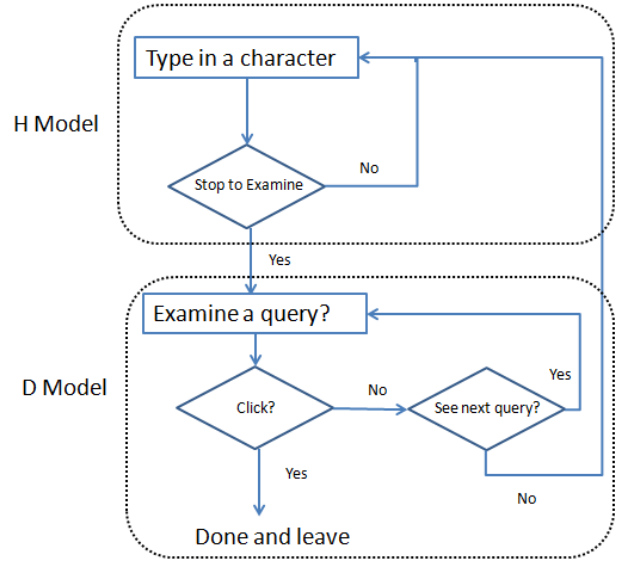
Figure 2: TDCM Flowchart
