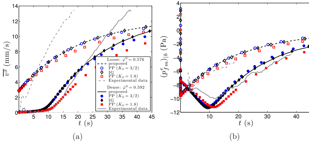
Figure 9: Low viscosity case: solid velocity \overline{v^x} and basal excess pore pressure (p_{fm}^e)_b for times t \in [10^{-2}\text{s}, 45\text{s}] , for the proposed model, the Pailha-Pouliquen model (with K_4 = 3/2 and K_4 = 1.8 ), the Iverson-George type model and the experimental data.
