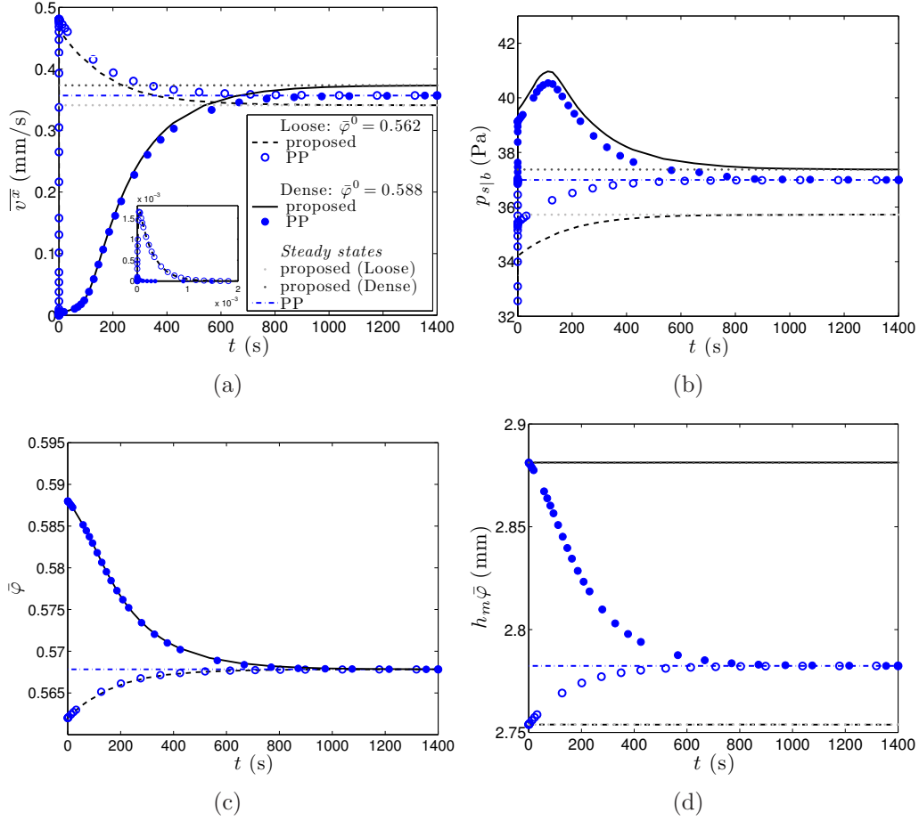
Figure 3: High viscosity case: simulated (a) solid velocity \overline{v^x} , (b) solid pressure p_{s|b} , (c) volume fraction \overline{\varphi} , and (d) h_m \overline{\varphi} . Horizontal dotted and dash-dotted lines represent the limit steady states. The relative velocity \overline{v^x} - \overline{u^x} is plotted in the insert of figure (a) (also in mm/s).
